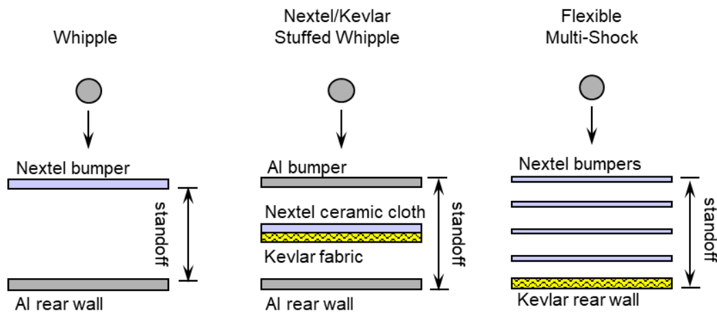
Fig. 1. Three different MMOD shield types using Nextel bumpers.
