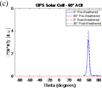
Fig. 2. The (a) reflectance spectrum and BRDF results at (b) 0° and (c) 60° angles of incidence for pre- and post-weathered GPS Solar Cell measured during Campaign #1.
