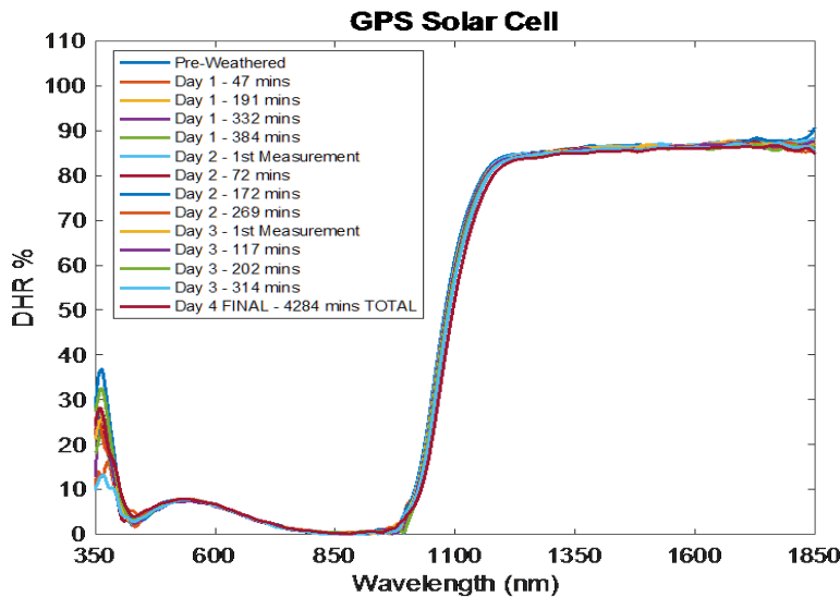
Fig. 2. The (a) reflectance spectrum and BRDF results at (b) 0° and (c) 60° angles of incidence for pre- and post-weathered GPS Solar Cell measured during Campaign #1.
