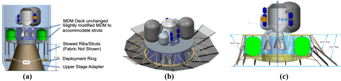
Figure 4. Additional details illustrated for ADEPT (a) launch configuration, (b) aerocapture and entry configuration with three flaps and (c) landed configuration to allow for cargo access.
