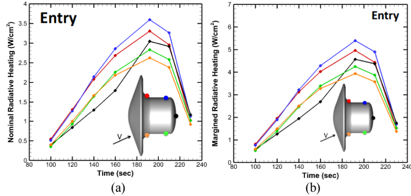
Figure 18. a) Unmargined radiative heating results on the aftbody; b) margined radiative heating.
