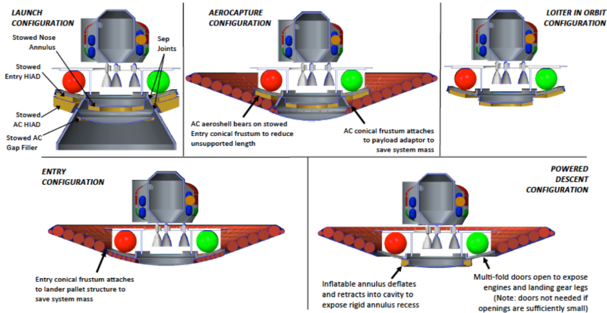
Figure 7. HIAD stowed and deployed configurations.
