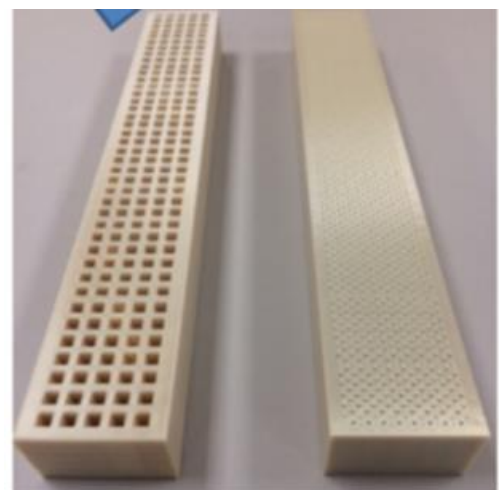
Acoustic Liner Test Articles
