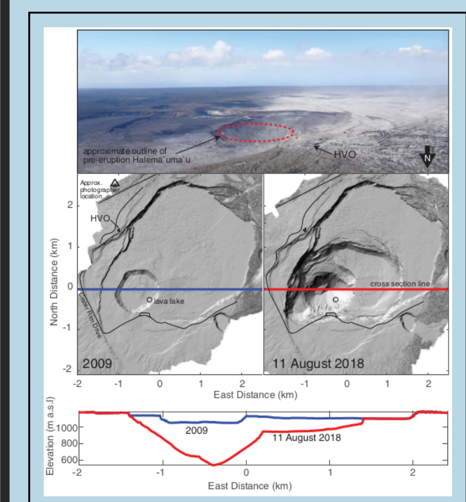
Figure (1) Lidar digital elevation models of the Kilauea summit crater after the 2008 (left) and 2018 (right) degassing events [9].
