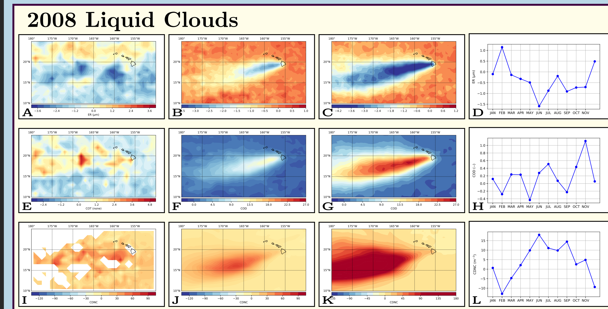
Figure (2) MODIS observations and GEOS-5 predictions for liquid clouds following 2008 Kilauea degassing event. From left: MODIS JJA anomaly wrt seasonal climatology (2003 – 2015), GEOS-5 prediction difference for 1 \times – 0 \times emissions, GEOS-5 model prediction difference for 5 \times – 0 \times emissions, MODIS monthly mean anomaly for 2008 with seasonal means removed. A-D: effective radius (microns), E-H: Cloud optical depth (COD; -), I-L: cloud droplet number concentration (CDNC; \text{m}^{-3} ).
