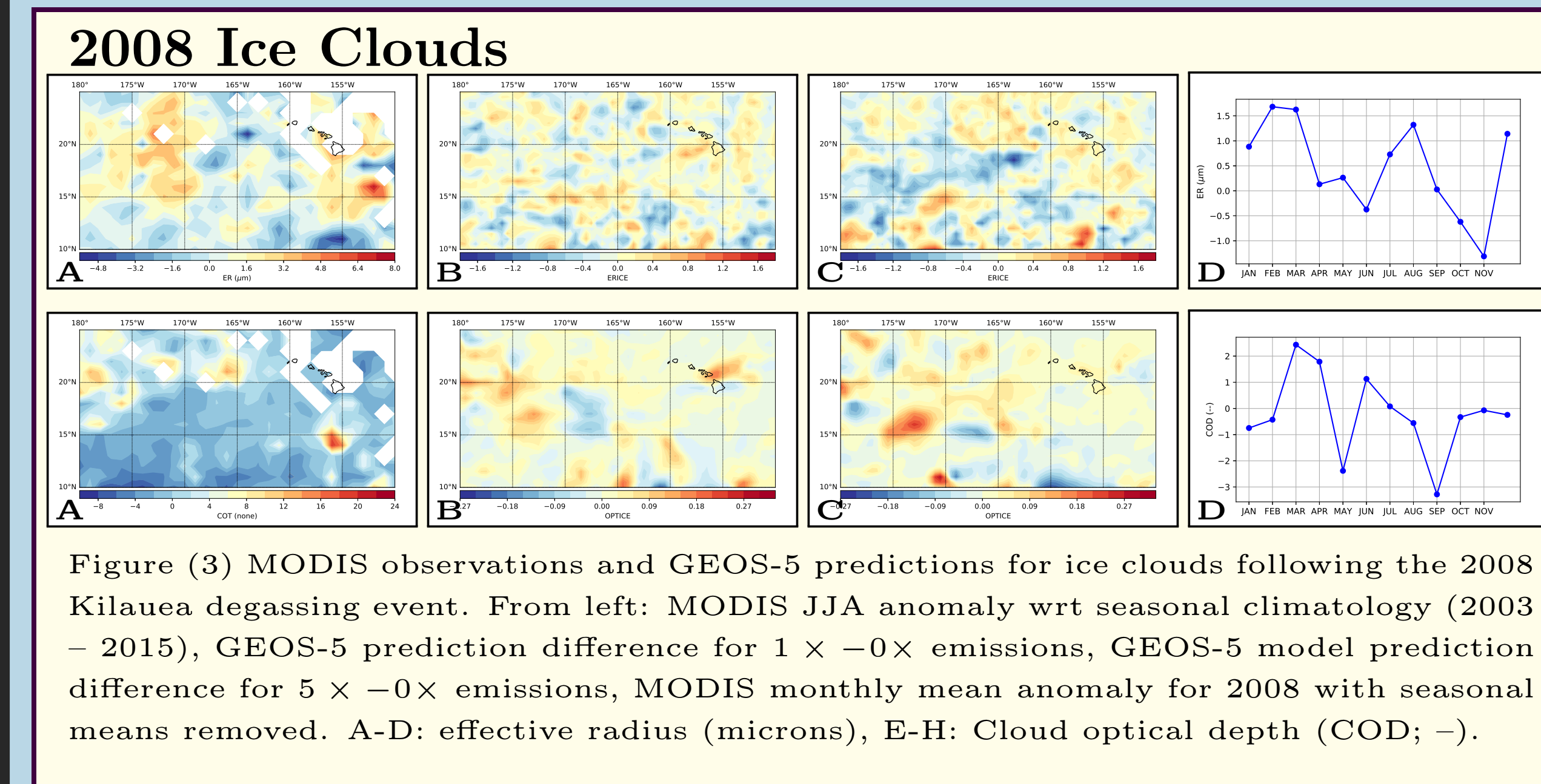
Figure (3) MODIS observations and GEOS-5 predictions for ice clouds following the 2008 Kilauea degassing event. From left: MODIS JJA anomaly wrt seasonal climatology (2003 – 2015), GEOS-5 prediction difference for 1 \times – 0 \times emissions, GEOS-5 model prediction difference for 5 \times – 0 \times emissions, MODIS monthly mean anomaly for 2008 with seasonal means removed. A-D: effective radius (microns), E-H: Cloud optical depth (COD; -).
