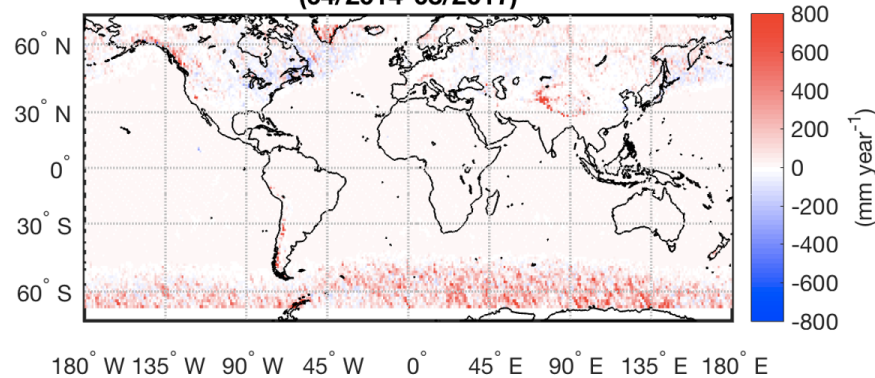
2C-SNOW-PROFILE (>8dBZ) - 2ADPR MS (T2m) Snowfall Difference (04/2014-03/2017)
