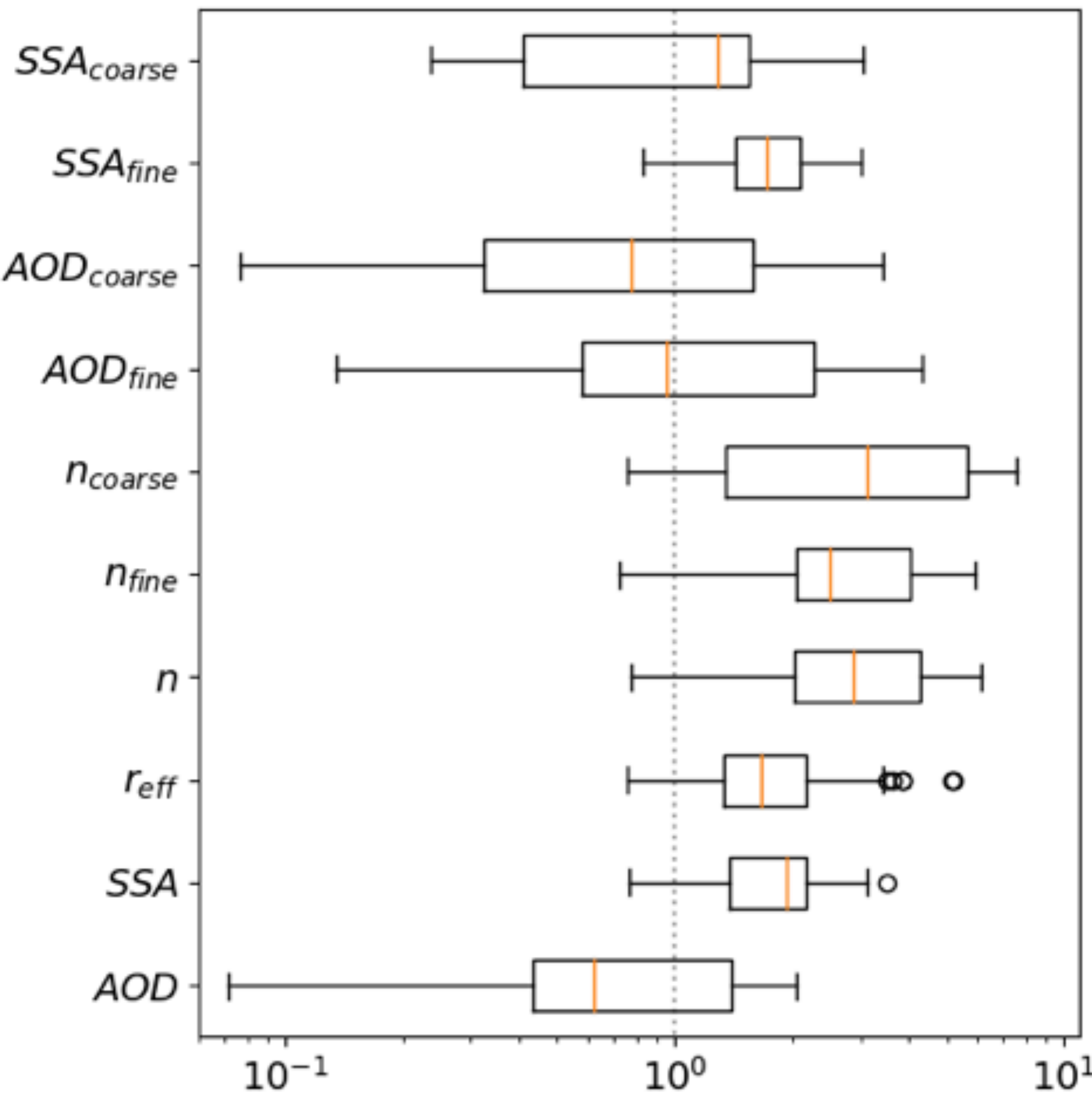
Figure 3: Relative assessment of expected polarimeter retrieval accuracies for aerosol simulations over a dark surface. The boxes extend from the lower to upper quartiles of the normalized errors, with the orange line representing the median. The whiskers show the full range of the data excluding outliers, which are represented by circles and consist of points that are more than 1.5 times the interquartile range above or below the upper or lower quartile, respectively. Values to the left of the dotted line meet the retrieval requirements, while those to the right exceed them.
