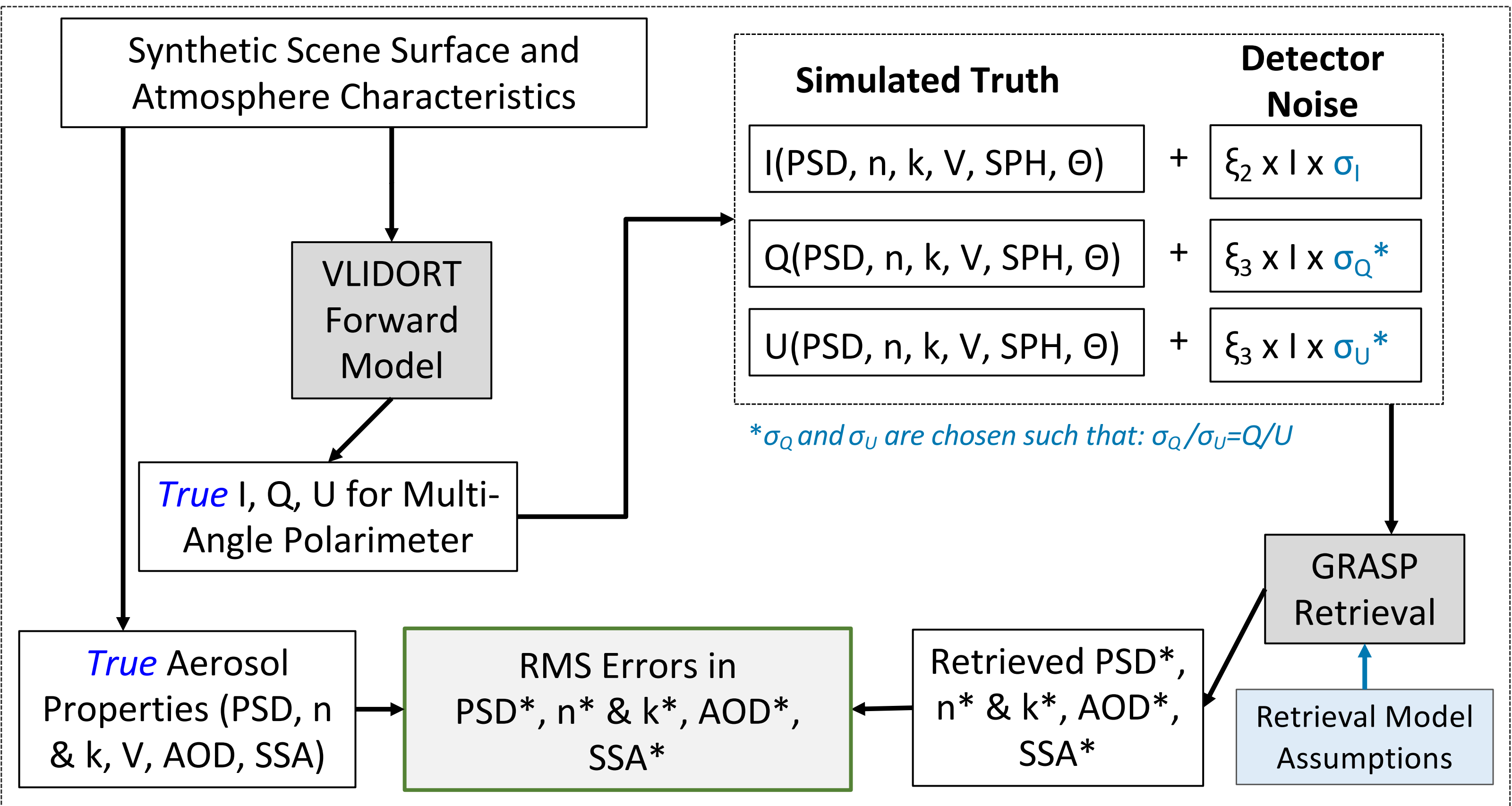
Figure 2: The workflow for the OSSE. Synthetic observations are generated with vertical profiles of G5NR atmospheric properties, and surface properties generated from either MODIS land BRDF observations, or wind driven ocean glint models. These inputs are fed into the VLIDORT radiative transfer model to produce a TOA I, Q, and U values. These are perturbed by a random value \xi multiplied by the instrument radiometric uncertainty \sigma . This I, Q, and U are fed into the GRASP retrieval algorithm, and the retrieved aerosol properties are compared to the True aerosol properties used to generate the synthetic observations.
