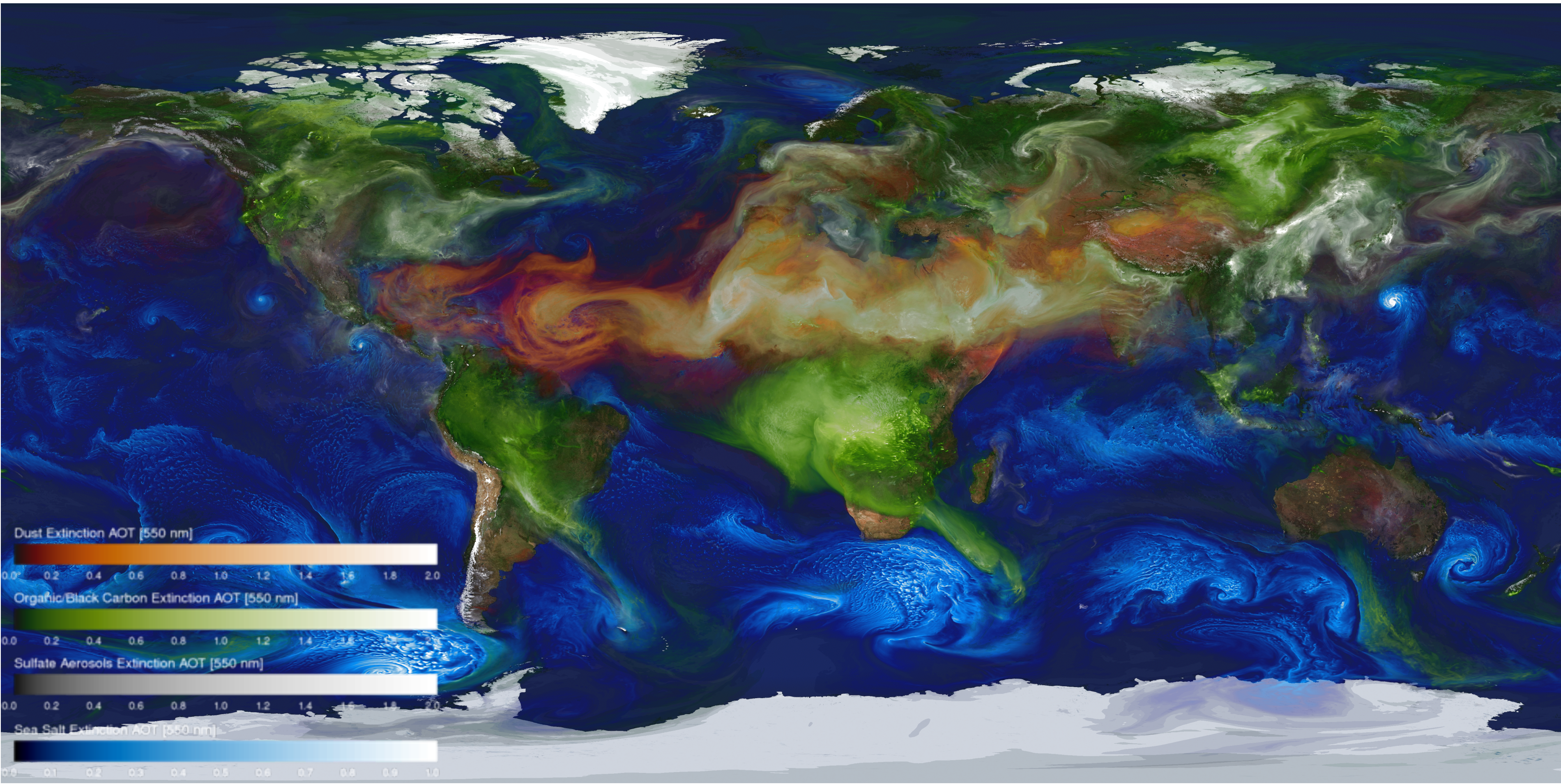
Figure 1: The GEOS-5 Nature Run (G5NR) is a 1.5 year high resolution (7 km) free-running mesoscale simulation that was produced by the Global Modeling and Assimilation Office (GMAO) to support mission planning studies. The G5NR provides a full meteorological description of the atmosphere as well as vertical profiles of concentrations of 15 aerosol species, CO, CO 2 , and O 3 at 30 minute time intervals. The G5NR forms the basis of the Observing System Simulation Experiment (OSSE).
