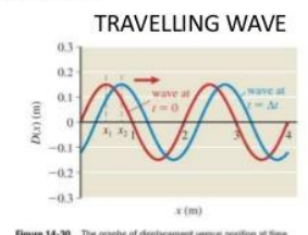
Figure 14-30 The graphs of displacement versus position at time t = 0 and t = \Delta t for a sinusoidal wave travelling from left to right.
