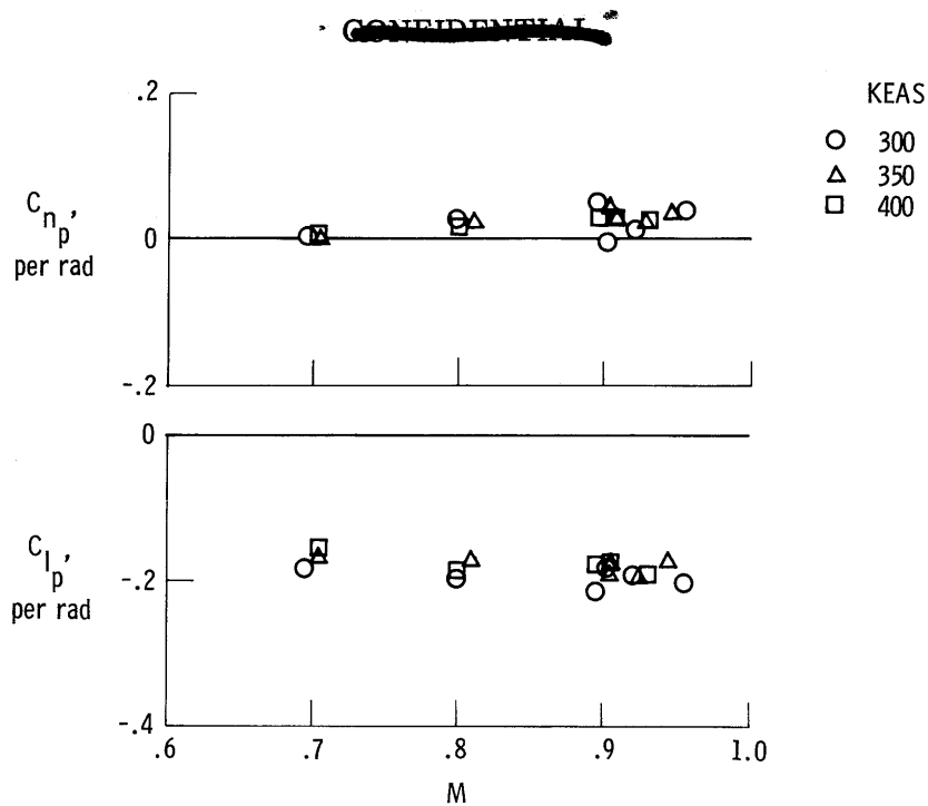
(b) C_{n_p}', C_{l_p}' . Flight data, camera pods on.
