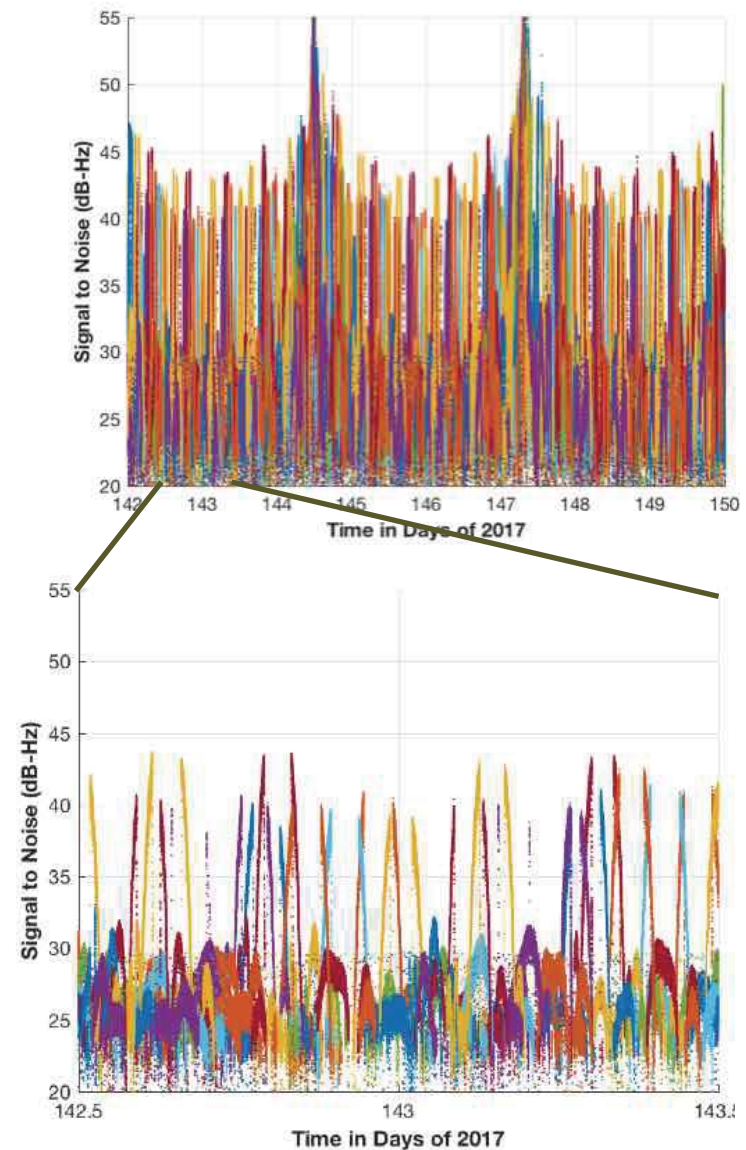
C/N 0 vs. time, near apogee
