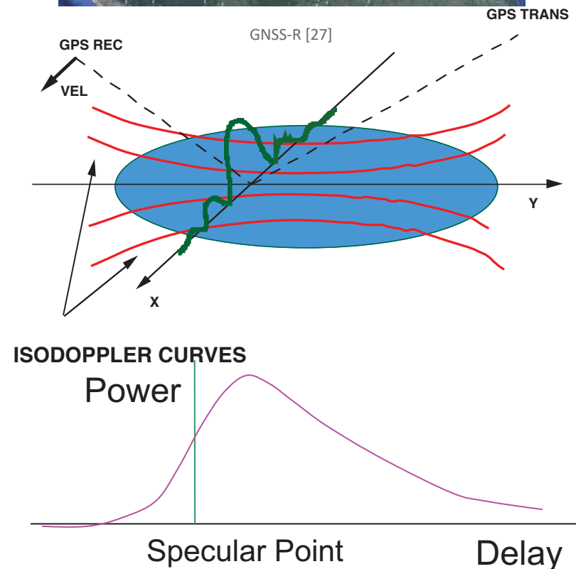
Reflected signal integrated along the Doppler coordinate: not a symmetric triangle [27]
