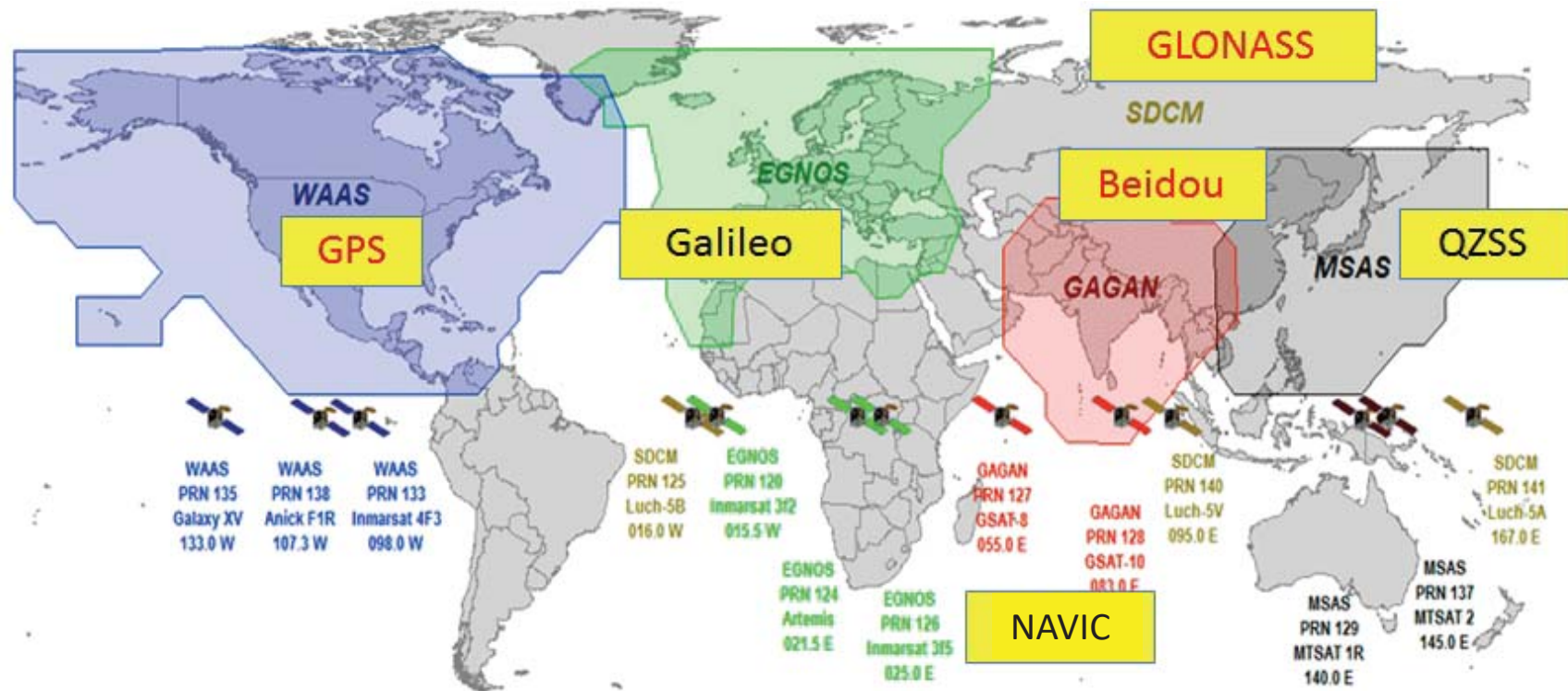
GNSS constellations, augmentations, and regional constellations [7]
