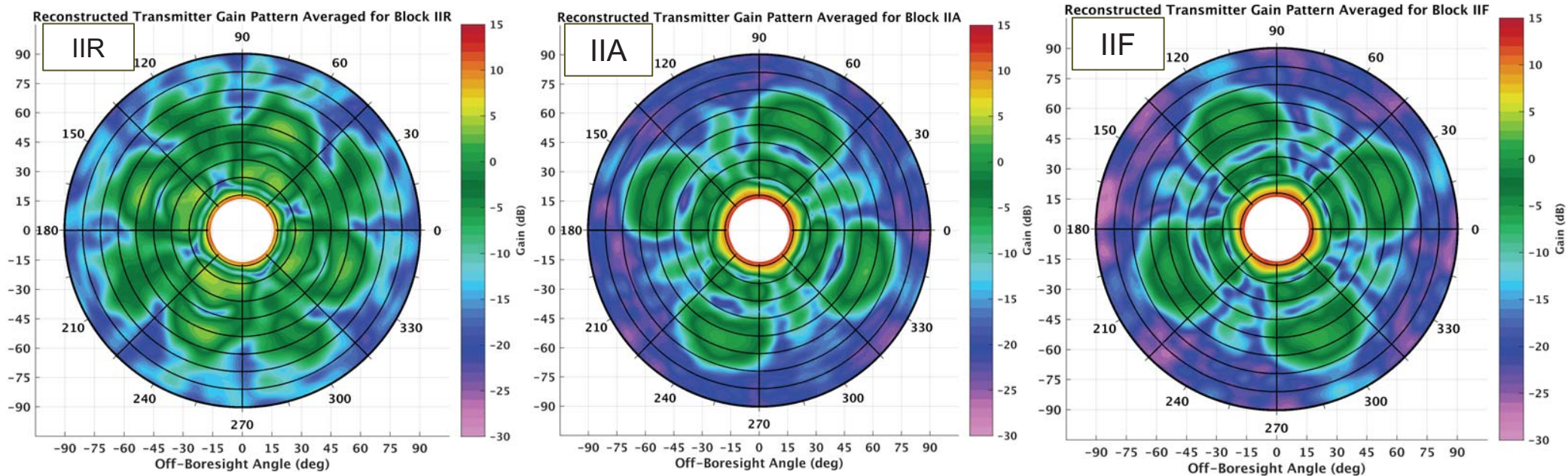
GPS Antenna Patterns from ACE [26]
