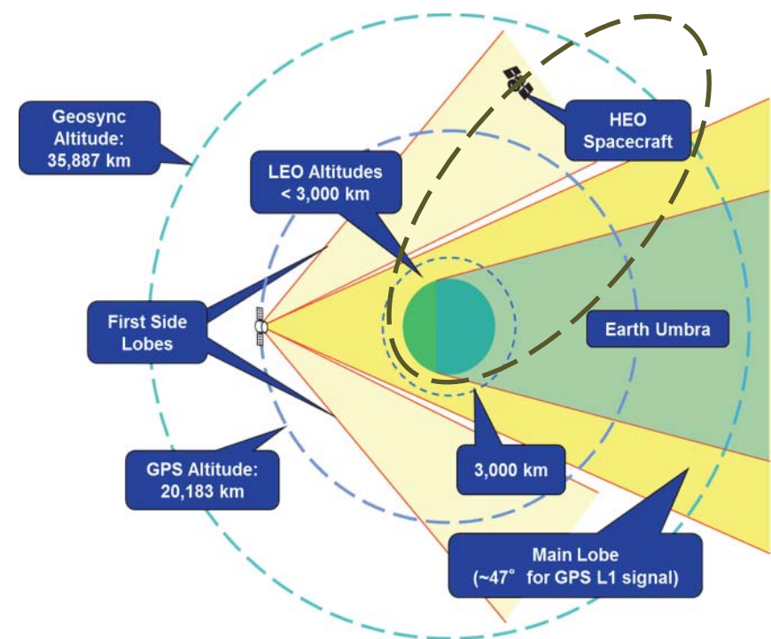
The Space Service Volume [25]
