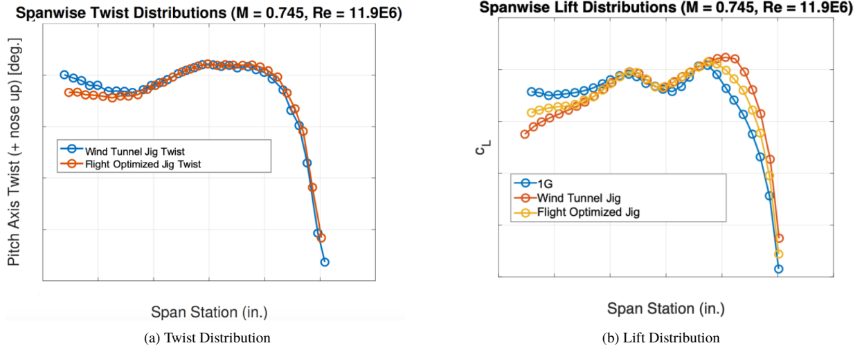
Figure 24 Drag Minimization Jig Twist Optimization Candidate
