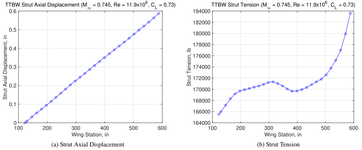
Figure 20 TTBW Strut Axial Displacement and Tension at Mach 0.745 and C_L = 0.73
