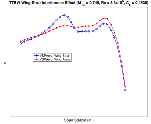
(b) Lift Coefficient Distribution - VSPAERO
