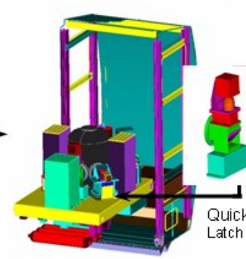
Step 4 Unstow/Install Payload Specific, Diagnostics/Electronics
