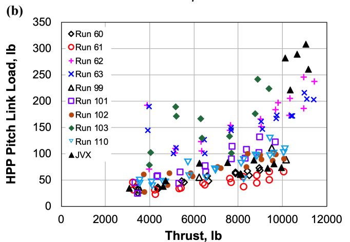
Fig. 13. TTR/699 unsteady pitch-link loads vs. thrust at M_{tip}=0.684 ; PTR/JVX data at M_{tip}=0.709 .
