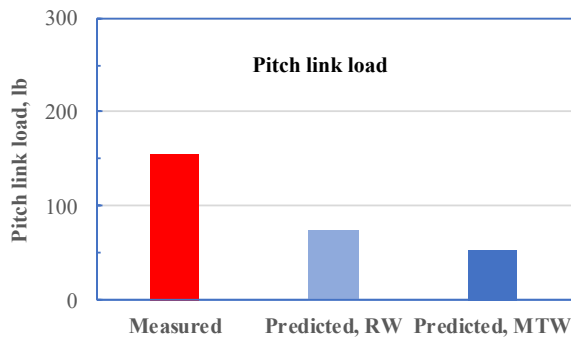
Figure 30. Measured and predicted hpp pitch link load, 60-deg yaw, \Omega=566 , V=92 knots, \mu=0.20 , C_T/\sigma=0.080 .
