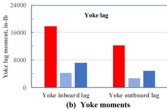
Figure 41. Measured and predicted blade and yoke hpp lag moments, 75-deg yaw, \Omega=573 , V=70 knots, \mu=0.15 , C_T/\sigma=0.081 .
