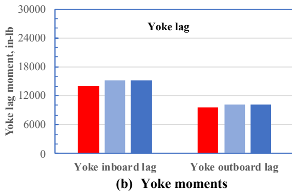
Figure 17. Measured and predicted blade and yoke hpp lag moments, 45-deg yaw, \Omega=568 , V=92 knots, \mu=0.20 , C_T/\sigma=0.080 .
