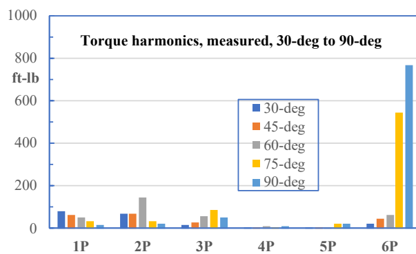
(a) Measured harmonics of torque
