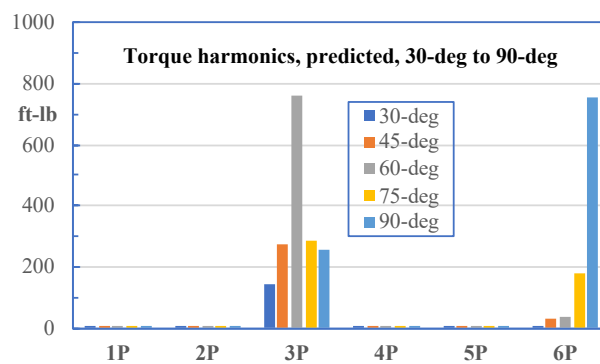
(b) Predicted harmonics of torque
