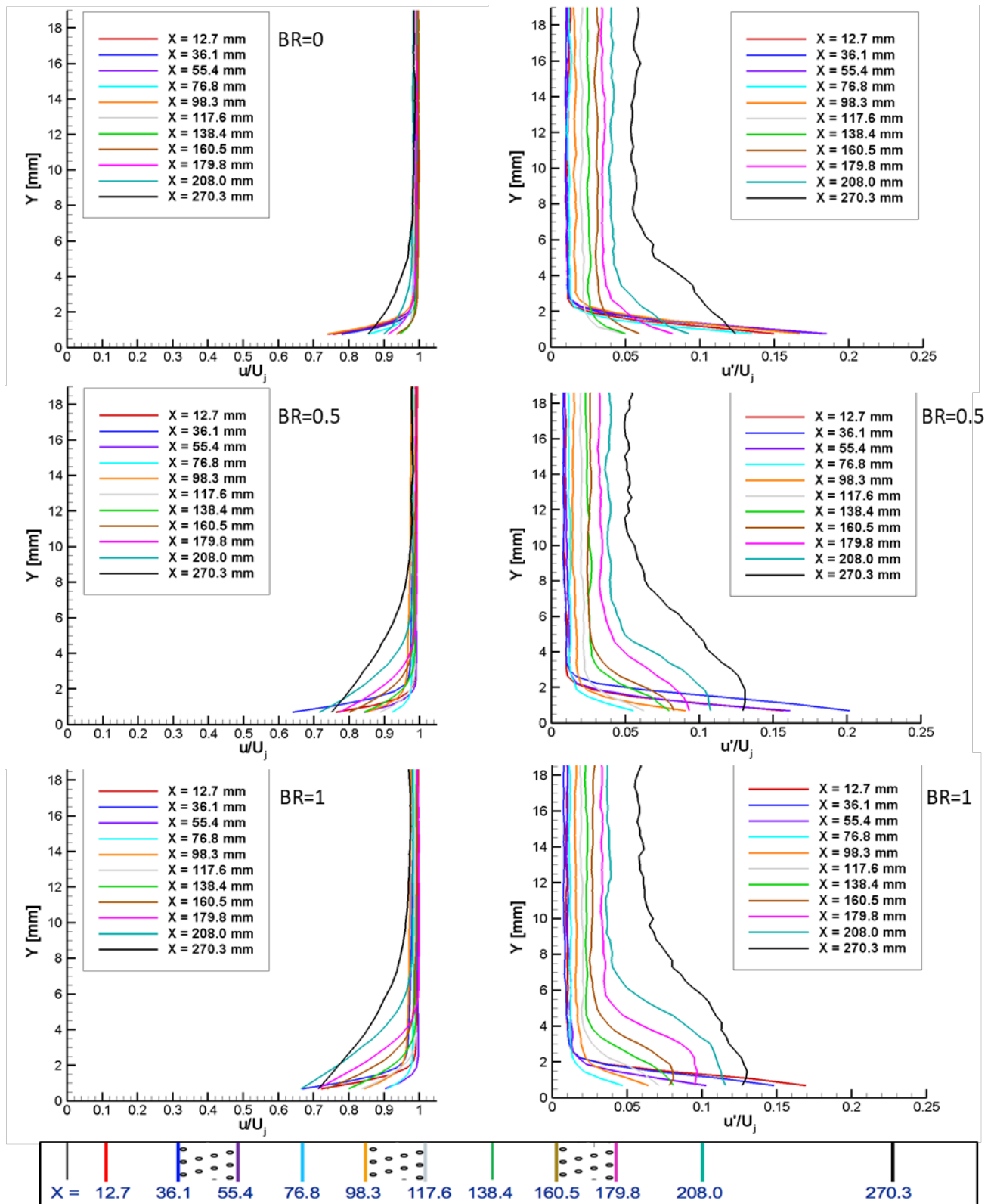
Figure 23. Streamwise PIV mean and rms velocity profiles along the centerline of the plate for Set Point 49 at BR=0 , 0.5 and 1 . The color coded key at the bottom shows the measurement stations along the plate where the measurements were collected.
