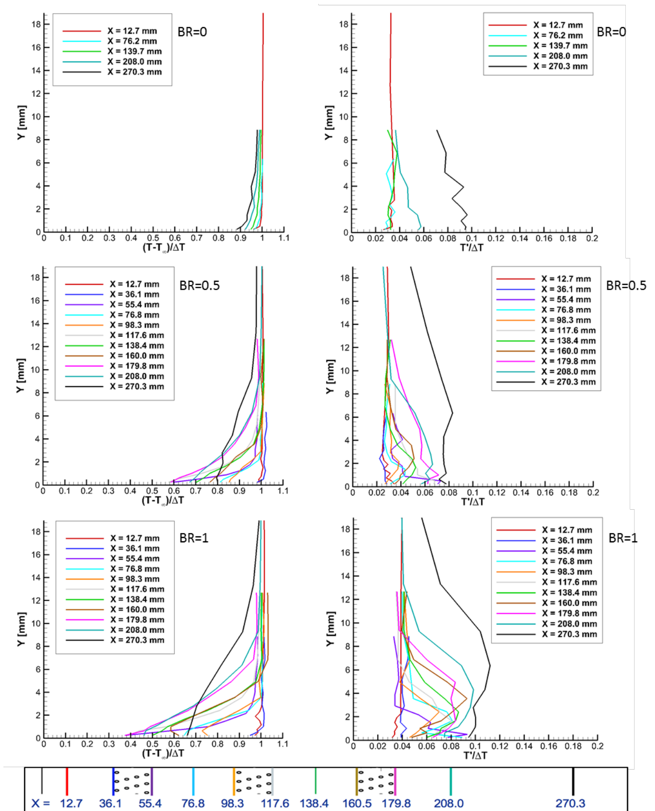
Figure 25. Raman mean and rms temperature profiles along the centerline of the plate for Set Point 49 at BR=0, 0.5, and 1. The color coded key at the bottom shows the measurement stations along the plate where the measurements were collected.
