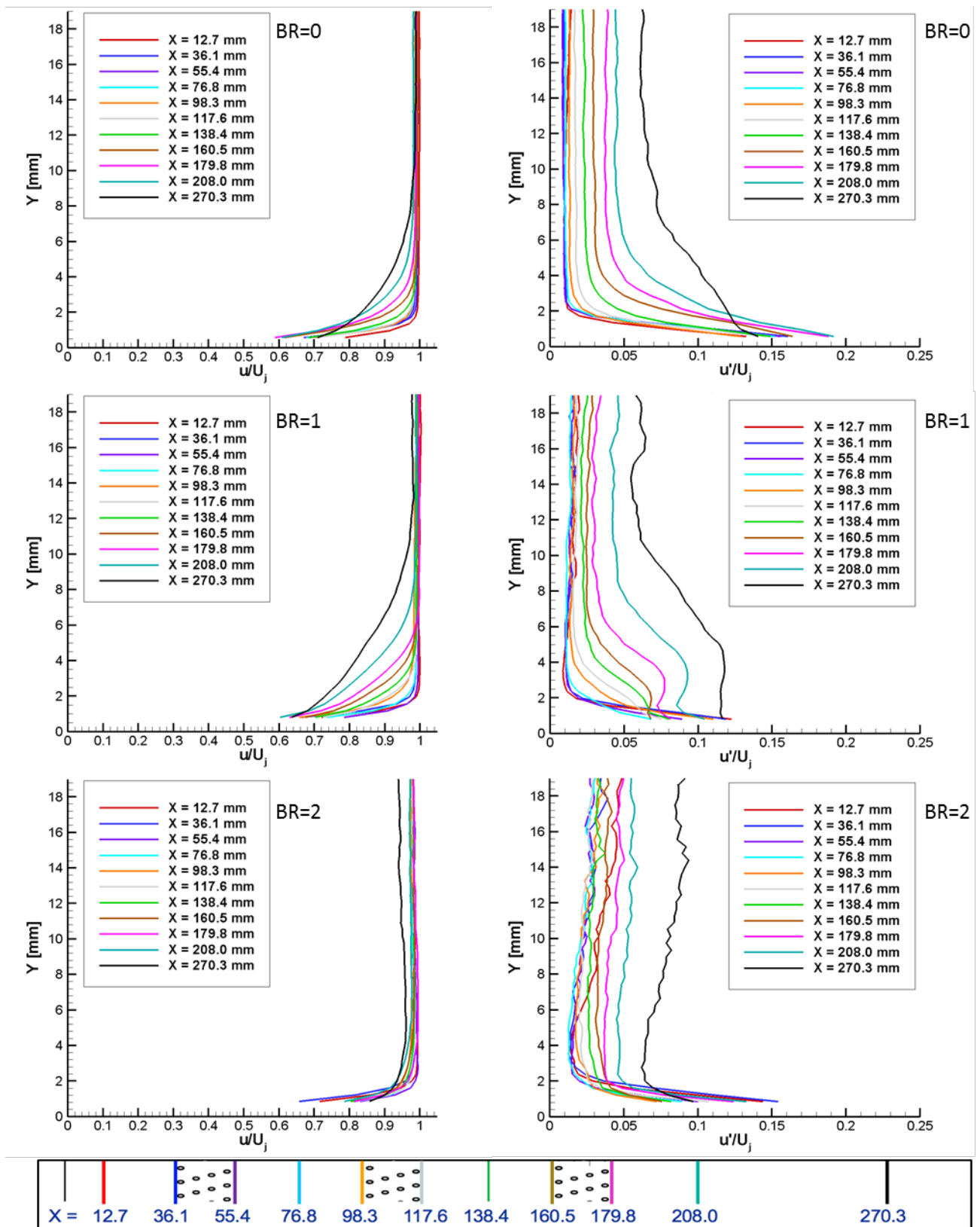
Figure 18. Streamwise PIV mean and rms velocity profiles along the centerline of the plate for Set Point 23 at BR = 0, 1 and 2 . The color coded key at the bottom shows the measurement stations along the plate where the measurements were collected.
