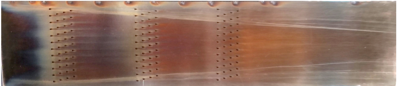
Figure 26. The perforated test plate which has discolored after several thermal cycles. The marks along the bottom edge are from zeroing the Raman laser relative to the model.
