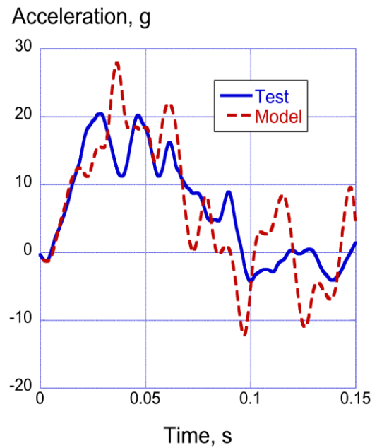
(b) Vertical acceleration.
