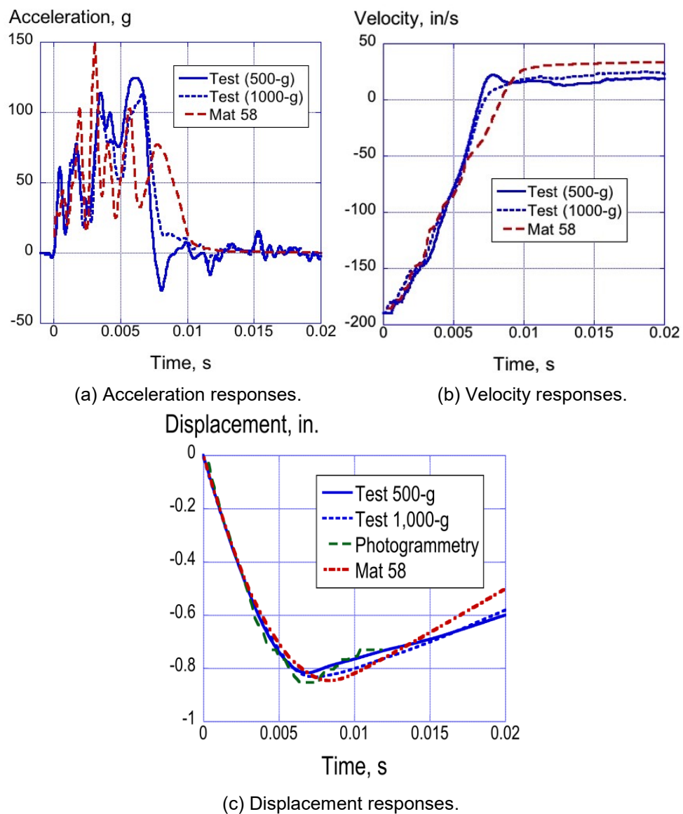
Figure 8.96. Experimental and Mat 58 analytical results for the I-beam 4-foot drop test [Fig. 86 of Jackson et al., 2014b].
