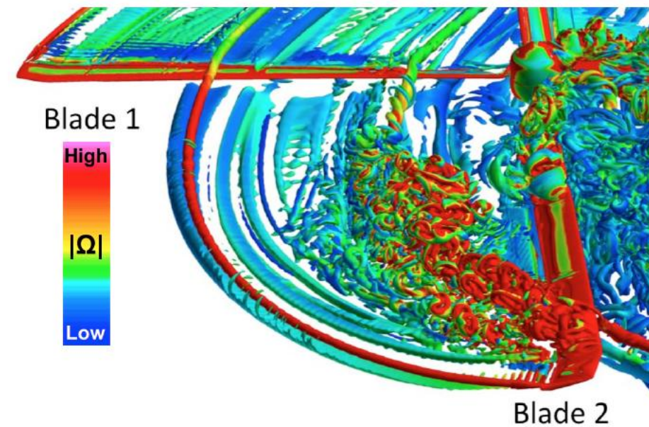
a) Blade 1 at \psi=180^\circ .
