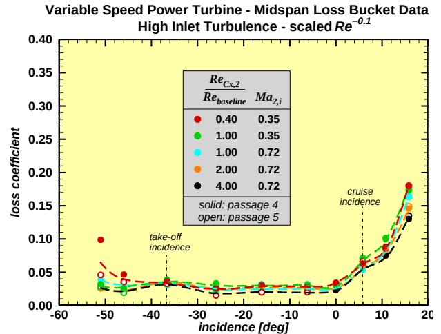
Figure 7.9. Re^{-0.1} scaled midspan loss vs. incidence—high Tu (Fig. 22b of Flegel et al. [2014]).
