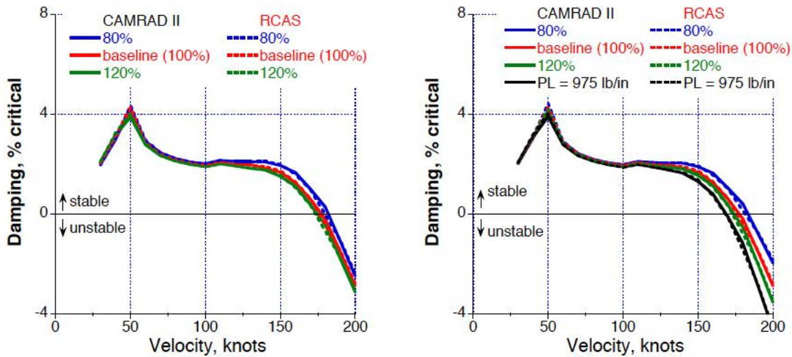
(a) Damping for flap stiffness variation. (b) Damping for pitch link stiffness variation. Figure 2.31. Damping of wing beam mode with yoke flap stiffness and pitch link stiffness variation (Yeo et al. [2017]).
