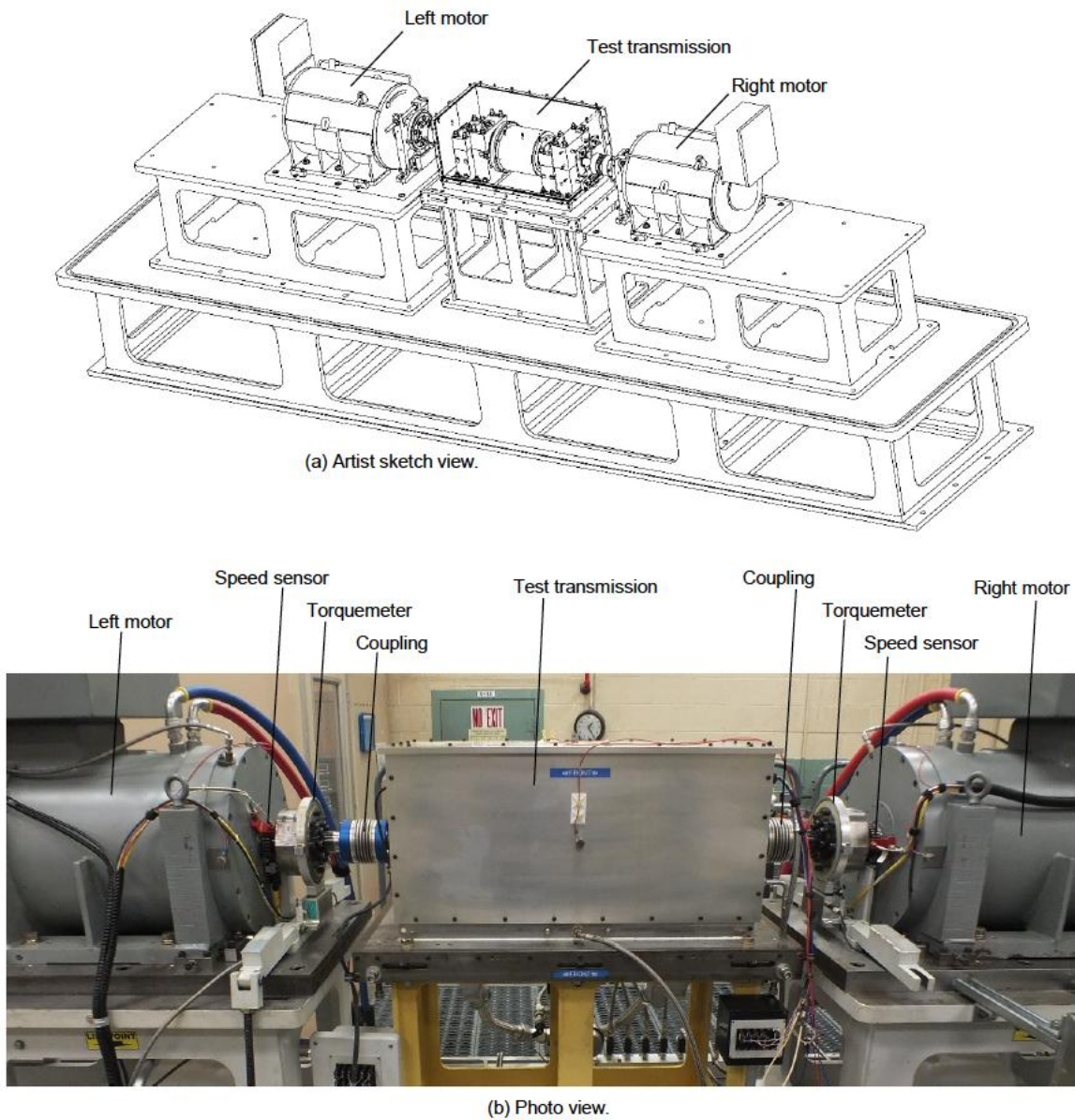
Figure 6.3. NASA GRC Variable-Speed Transmission Test Facility (Fig. 1 of Lewicki and Stevens [2015]).
