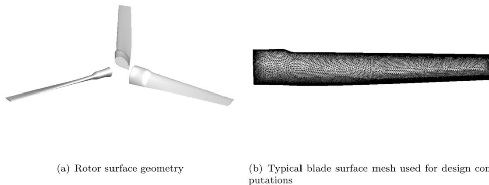
Figure 3.37. TRAM used in adjoint-based design optimization (Fig. 1 of Jones et al. [2014]).
