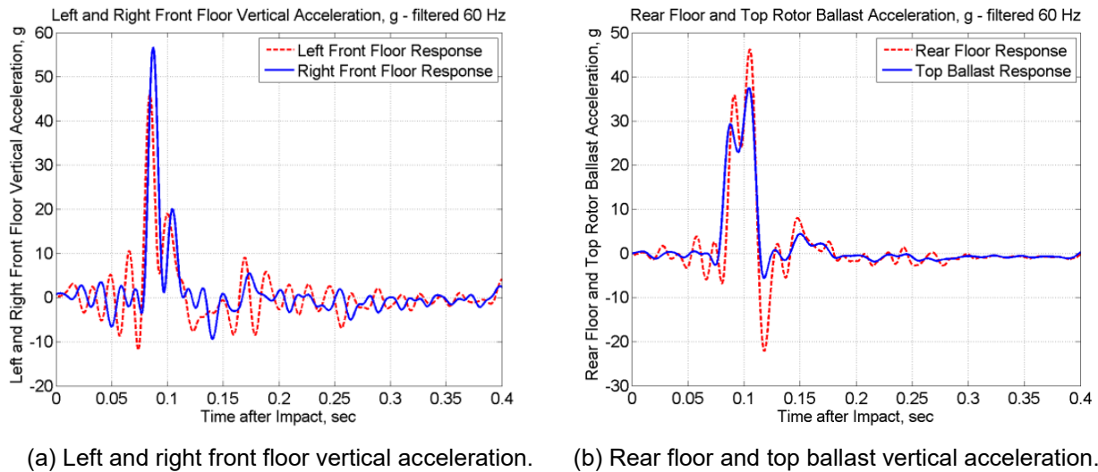
Figure 8.17. Measured acceleration time histories from the MD-500 crash test without DEA [Figs. 12 and 13 of Littell, 2011].
