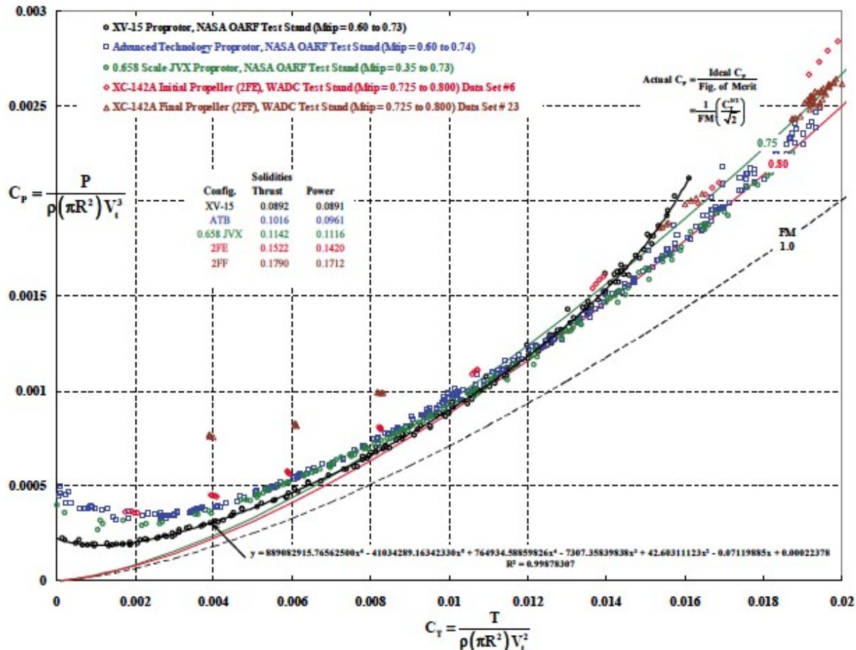
Figure 2.28. The thrust coefficient required to obtain optimum performance increases as solidity increases (Fig. 13 of Harris [2017]).
