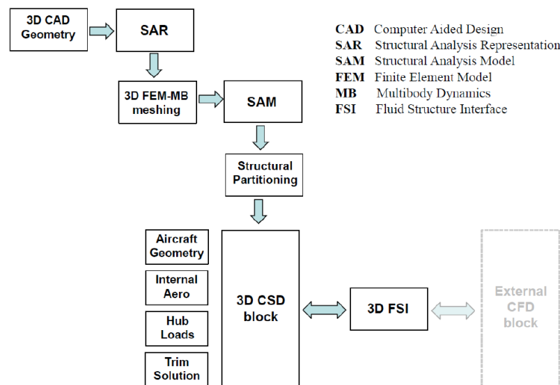
Figure 2.12. Integrated 3D workflow (Fig. 1 of Datta and Johnson [2014]).
