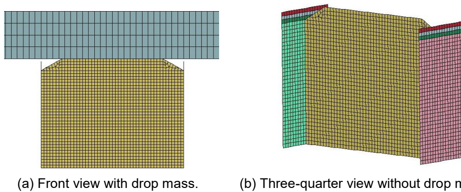
Figure 8.95. LS-DYNA model of the I-beam component [Fig. 83 of Jackson et al., 2014b].
