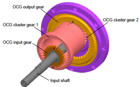
(b) 3D view of OCG gearing (region 1).
