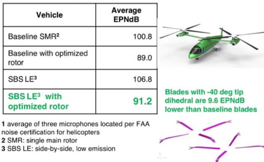
Figure 11.14. Comparison of predicted noise metrics 1 for FAA descent condition required for noise certification.
