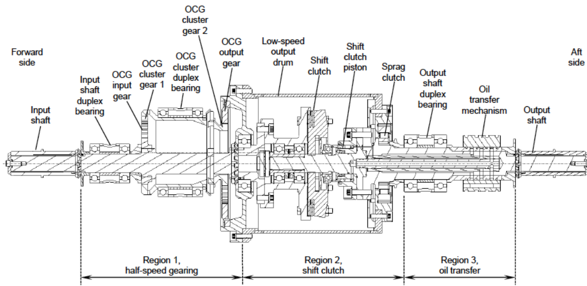
(a) Cross-sectional view.
