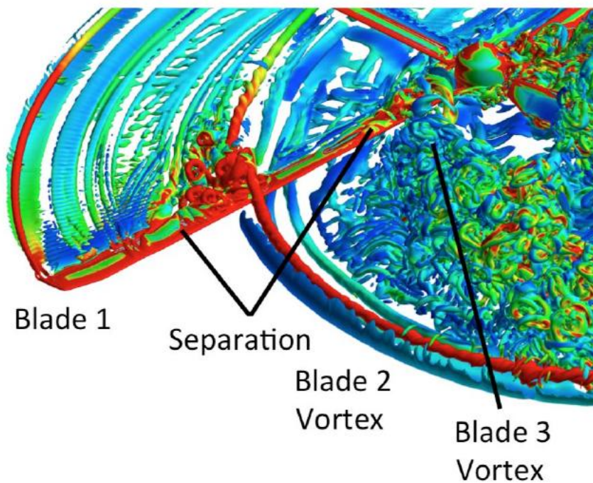
b) Blade 1 at \psi=225^\circ .
