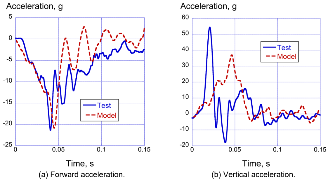
Figure 8.57. Forward and vertical test and analysis acceleration time histories at right side FS350 [Fig. 43 of Jackson et al., 2015].
