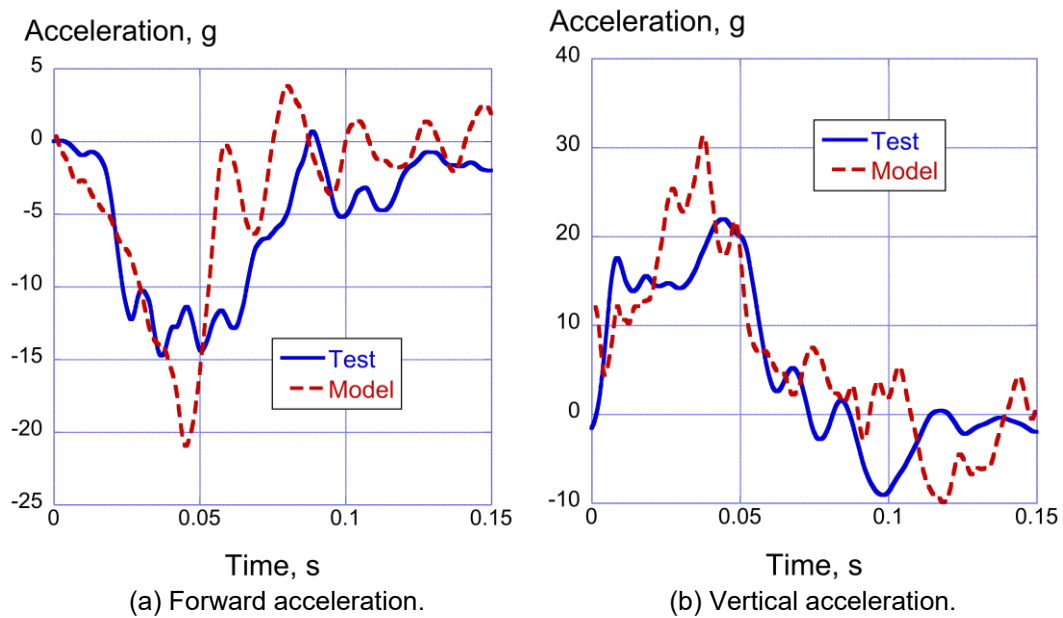
Figure 8.58. Forward and vertical test and analysis acceleration time histories at left side FS410 [Fig. 44 of Jackson et al., 2015].
