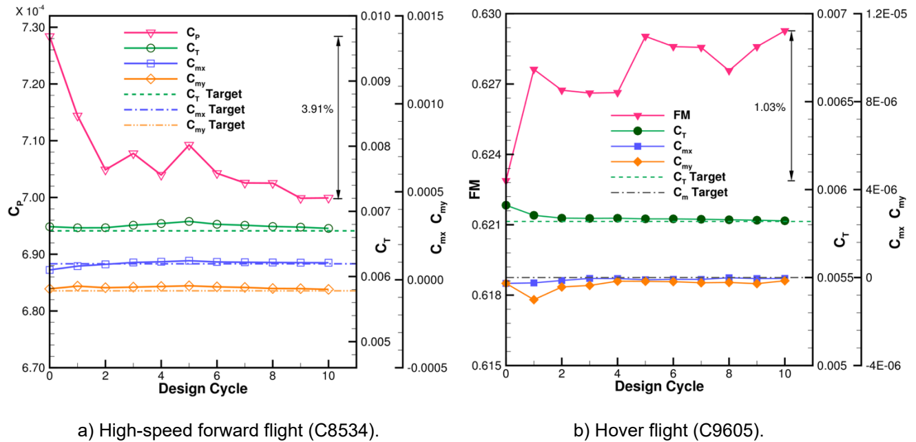
Figure 2.14. Multipoint UH-60A rotor design optimization using DYMORE/FUN3D toolset (Fig. 9 of Wang et al. [2019a]).
