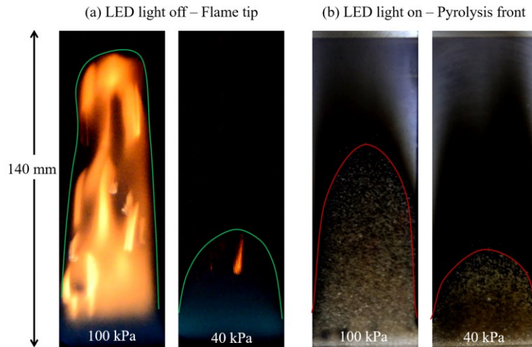
Figure 5: Front view of two representative frames at 100 and 40 kPa with (a) the light off showing the flame tip, and with (b) the strobe light on showing the pyrolysis front. All frames are taken 100 s after ignition.
