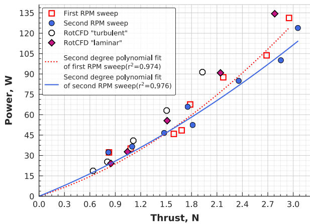
Figure 37. Experiment vs. simulations: plot of power vs. thrust for the two-bladed rotor at 10.7 mbar.
