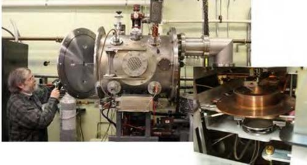
Lunar Dust Adhesion Bell Jar
