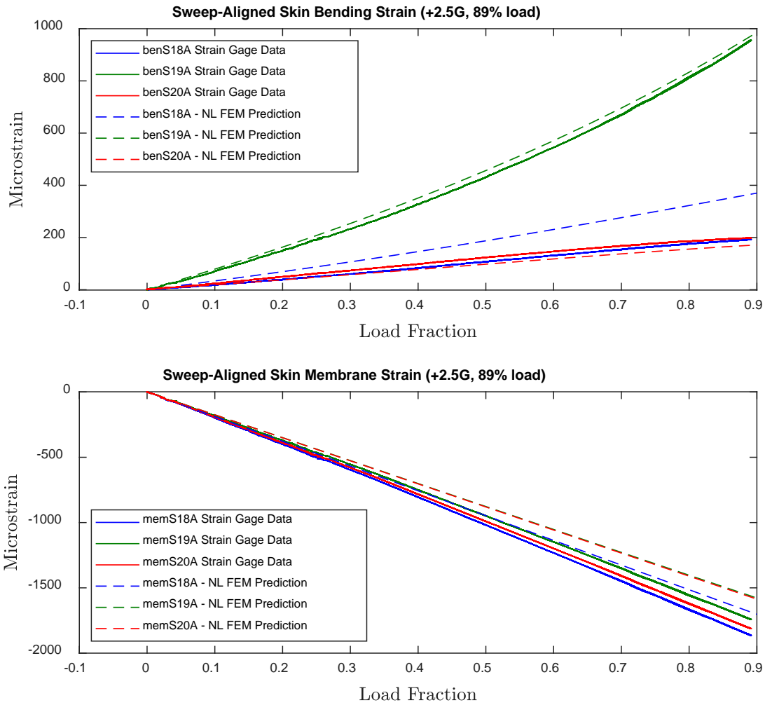
Figure 7.21. Bending and membrane strains for skin bays 18-20.
