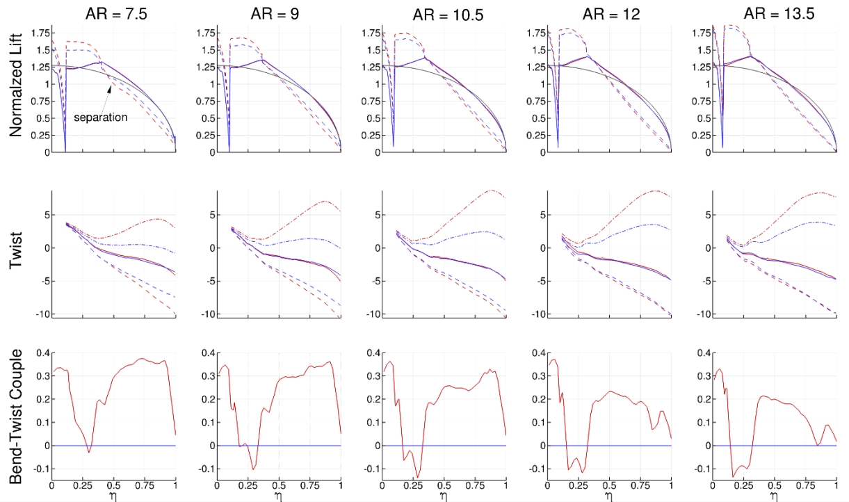
Figure 3.20. Passive load alleviation trend for increasing aspect ratio; tow-steered design (red), conventional design (blue).
