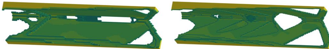
(a) Design obtained using 24 processors for mesh with 525,987 degrees of freedom.
