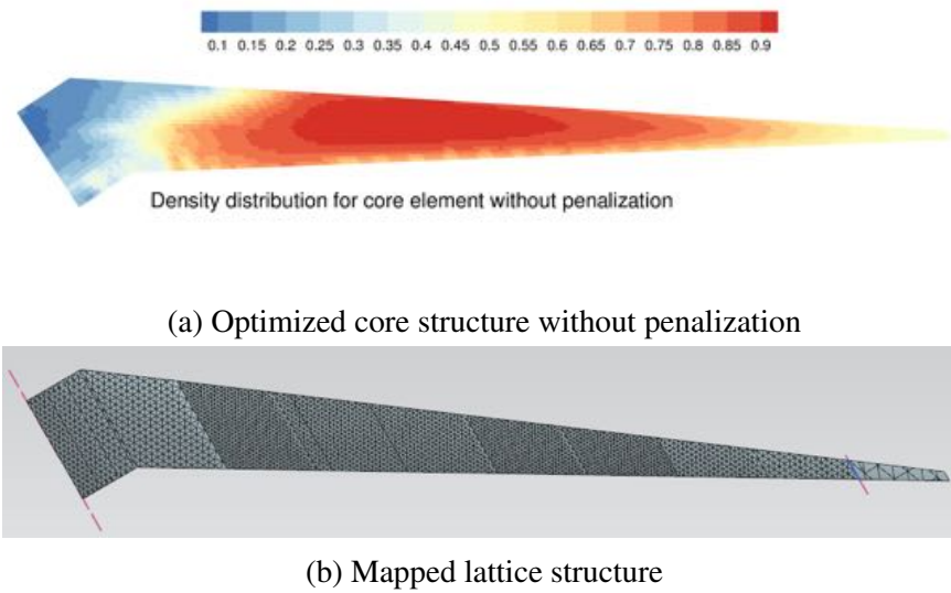
Figure 24: Comparison between the original core structure and the mapped lattice structure
