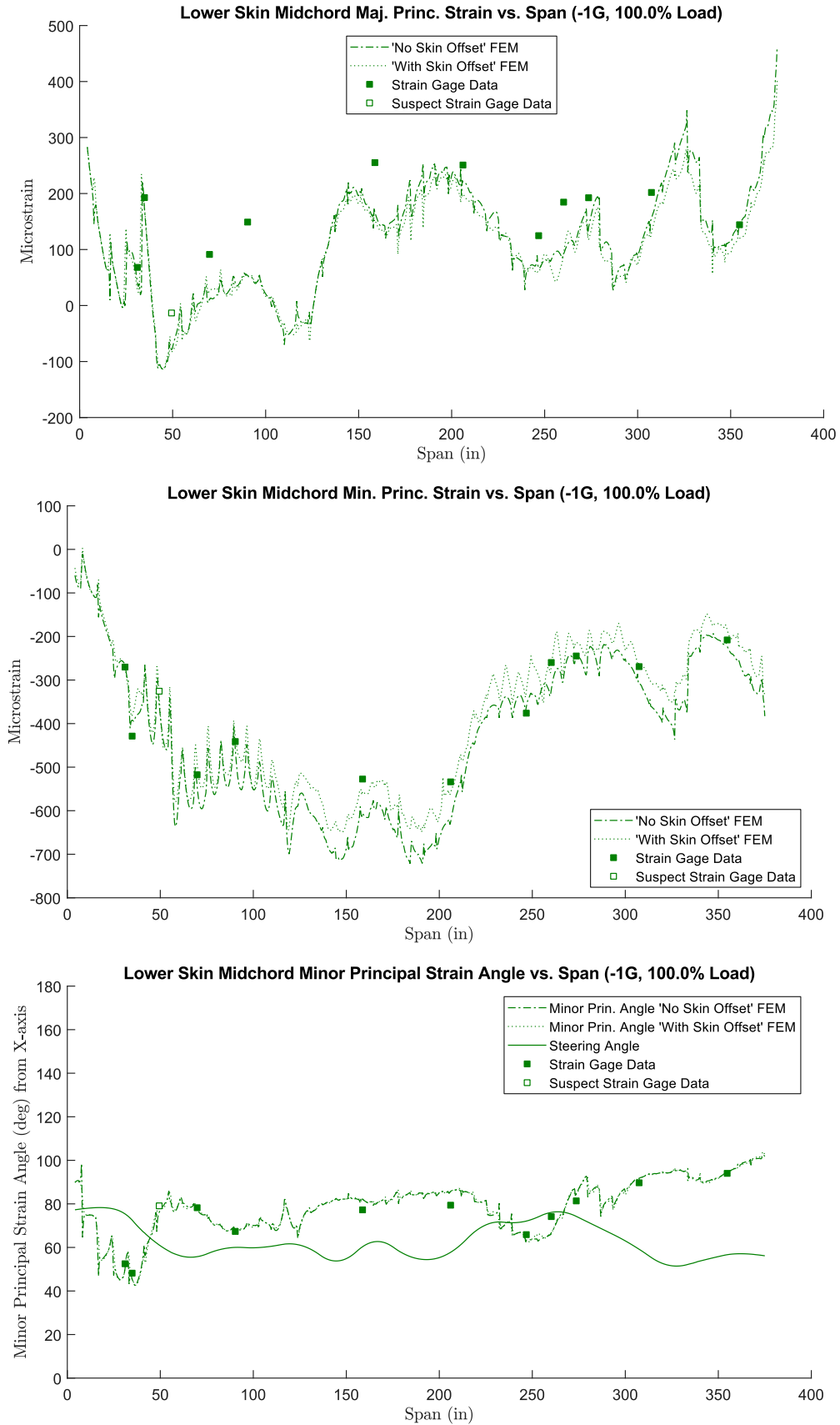
Figure C.29. Principal strains for lower skin mid-chord, -1G: major, minor and minor angle.
