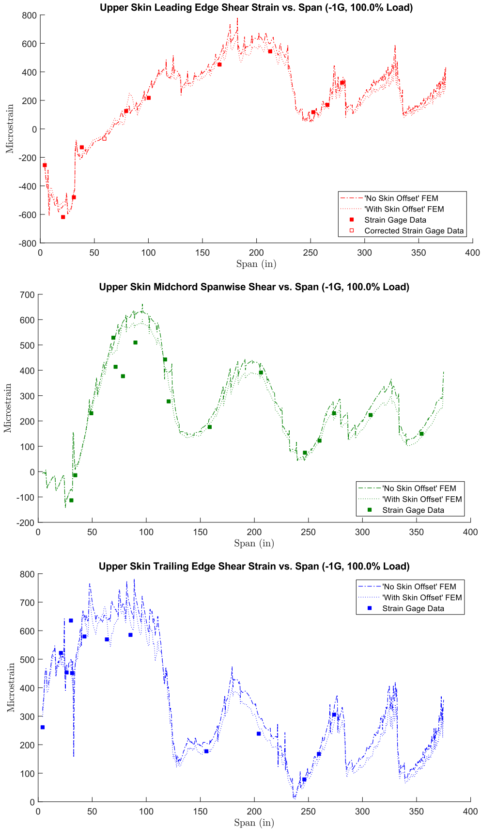
Figure C.13. Upper skin shear strains for -1G load case for leading edge (top), midchord (middle) and trailing edge (bottom).
