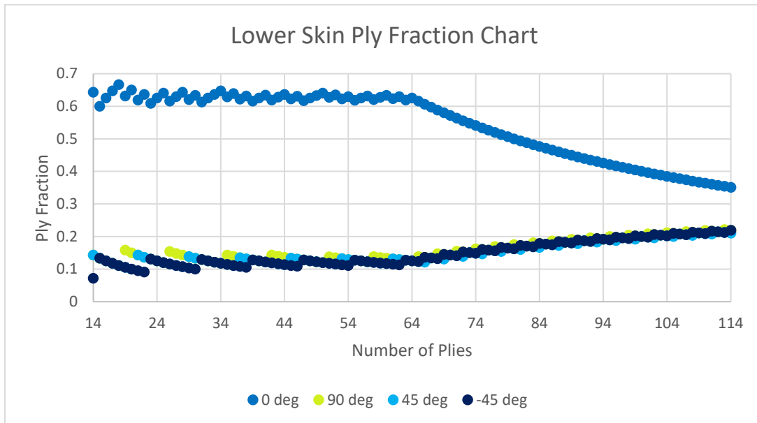
Figure 4.9. Lower skin ply fraction chart.
