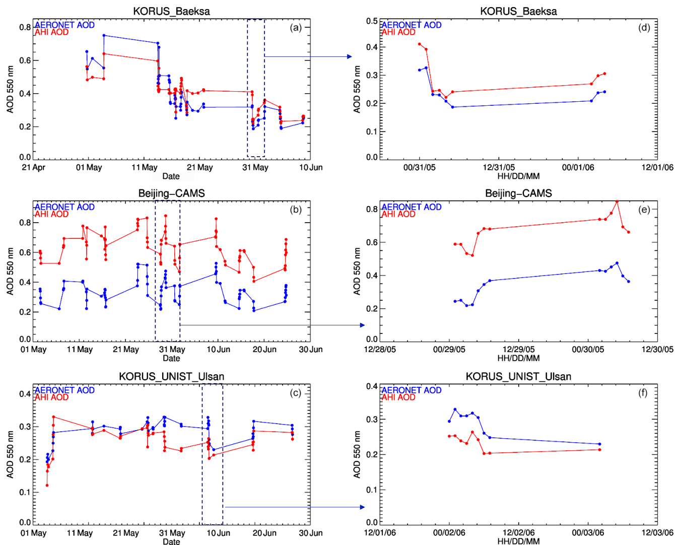
Figure 8. The time series of spatiotemporal mean AODs from AERONET (blue) and AH1 (red) for each hour of observation during the KORUS-AQ field campaign for the same three stations as shown in Fig. 7 (a–c). (d–f) Zoom of selected days as shown in the box with dotted lines in the left panels for each station.
