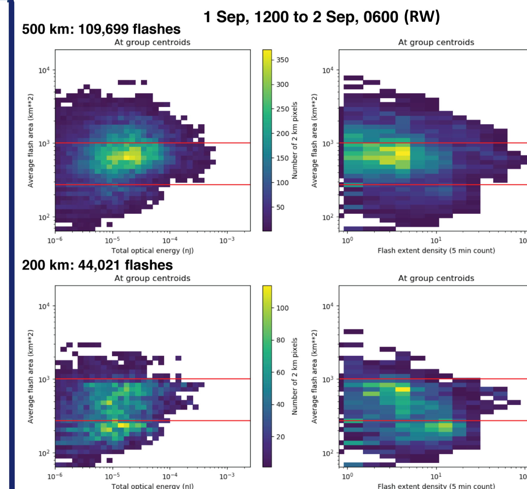
Fig. 3. As in Fig. 2, but for the first 18 hours of the period denoted "RW" in Fig. 1.
