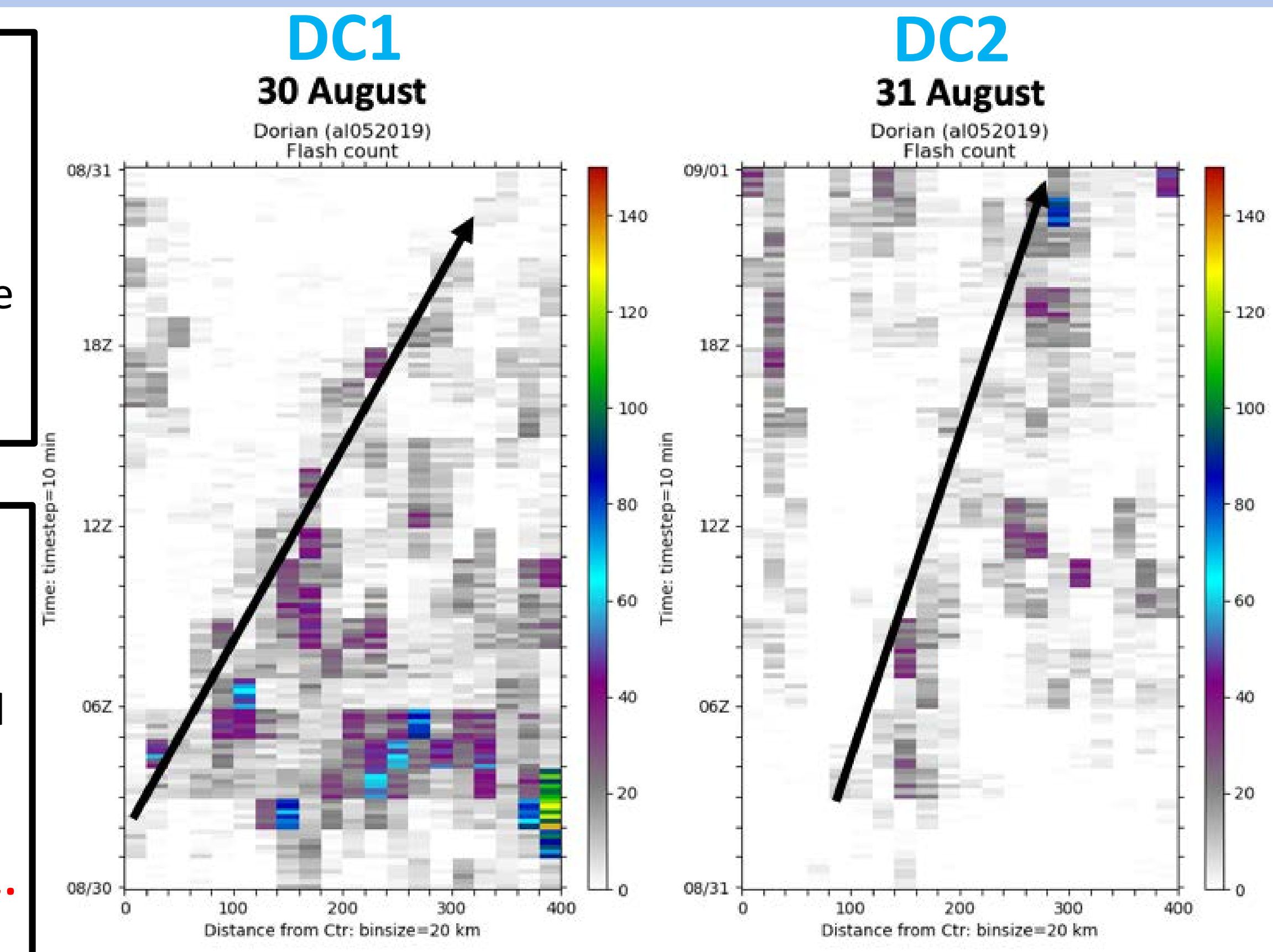
Fig. 6. Radius-time diagrams of GOES-16 GLM flash counts summed over 10-minute intervals in Hurricane Dorian for the periods indicated by "DC1" and "DC2" in Fig. 1. Black arrows denote an outward propagating region of lightning.
