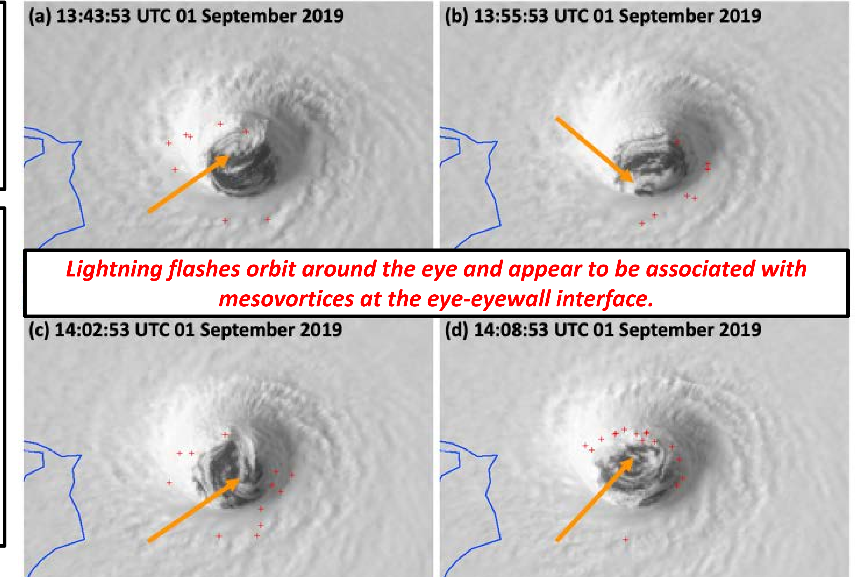
Fig. 4. GOES-16 ABI Channel 2 visible imagery of Hurricane Dorian with GLM flash locations (red marks) aggregated over two-minute periods centered on the time of the ABI image. Orange arrows denote the location of a mesovortex orbiting near the eye-eyewall interface.
