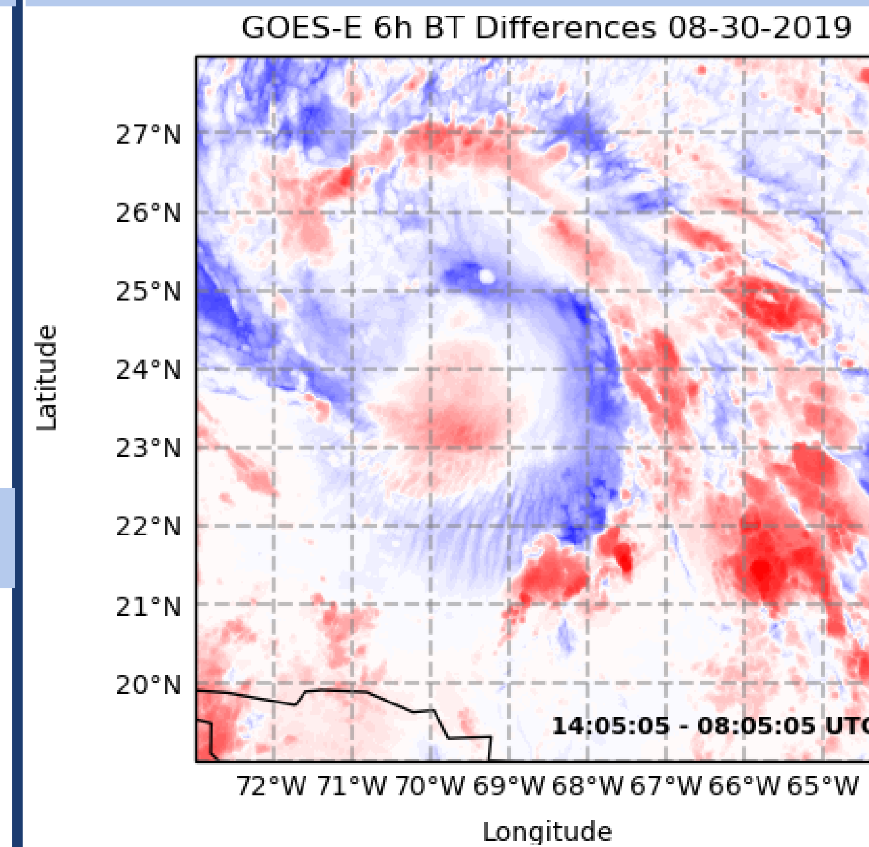
Fig. 5. GOES-16 ABI Channel 13 brightness temperature differences computed over a six-hour period. Red shading denotes warming temperatures over the 6-hour period and blue shading indicates cooling temperatures.
