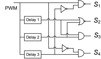
Fig. 16. Control logic implementation for CSG.
