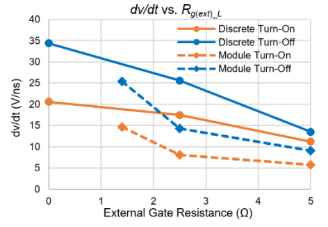
Fig. 9. Comparison of tested dv/dt between discrete device and power module.
