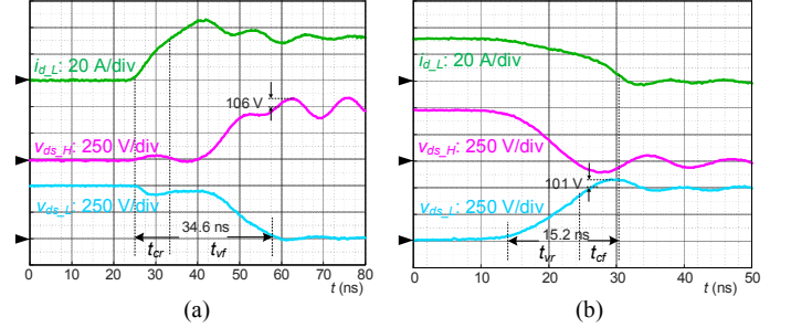
Fig. 5. Tested switching waveforms of discrete device when V_{DC}=500 V, I_o=30 A and R_{g(ext)_L}=0 \Omega . (a) Turn-on transient. (b) Turn-off transient.
