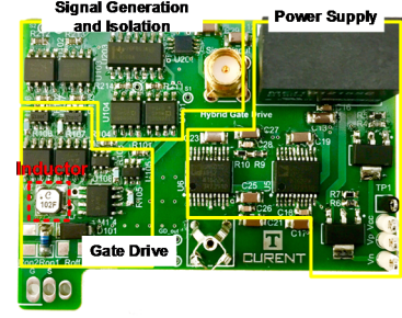
Fig. 19. Prototype of proposed CSG.
