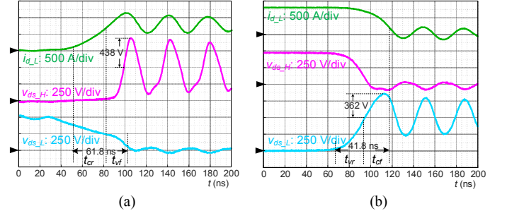
Fig. 6. Tested switching waveforms of discrete device when V_{DC}=500 V, I_o=30 A and R_{g(ext)_L}=0 \Omega . (a) Turn-on transient. (b) Turn-off transient.
