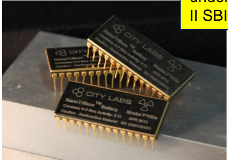
Chip-sized betavoltaic power sources manufactured by City Labs
