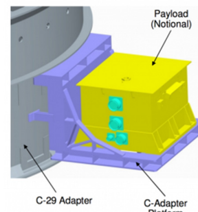
Figure 10.39: CAP. Image courtesy of ULA.
