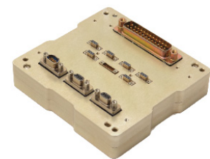
Figure 3.14: Clyde Space Small Satellite 3G FlexU EPS. Image courtesy of Clyde Space.
