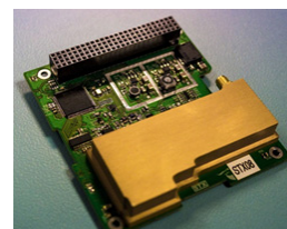
Figure 9.8: CubeSat-compatible S-band transmitter, to be used with either amateur or commercial bands. Image courtesy of Clyde Space Ltd.
