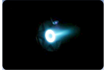
Figure 4.16: BHT-200 during operation. Image courtesy of Busek Co Inc.
