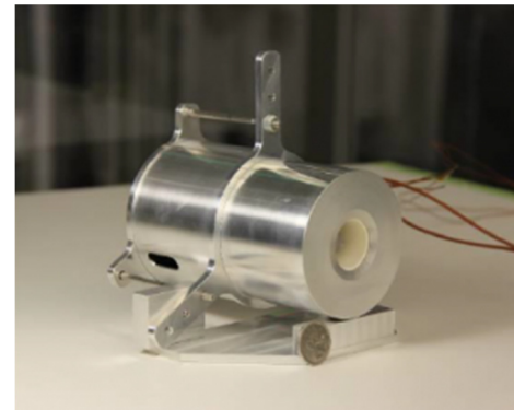
Figure 4.17: Cylindrical Hall Effect Thruster. Image courtesy of UTIAS SFL.
