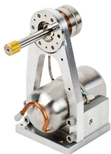
Figure 7.14: CryoTel DS1.5 1.4 W Cryocooler. Image courtesy of Sunpower, Inc. (2015).
