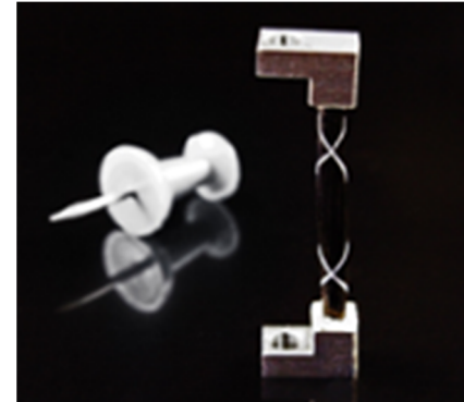
Figure 7.3: Graphite Fiber Thermal Straps (GFTS). Image courtesy of Thermal Management Technologies (2015).
