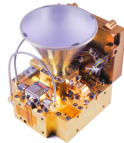
Figure 9.12: Ka-band transmitter with a horn antenna. Image courtesy of Astro Digital.
