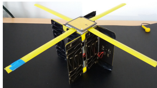
Figure 2.11: Unicorn-1 PocketQube. Image courtesy of Alba Orbital.
