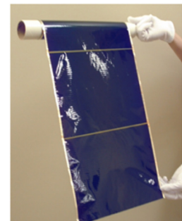
Figure 3.18: A series-connected string of production-sized cells on 1 mil polymer partially rolled onto a tube. Image courtesy of Casey (2014).
