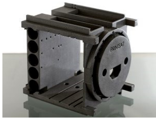
Figure 6.13: Windform PrintSat Structure. Image courtesy of CRP Technology (2015).
