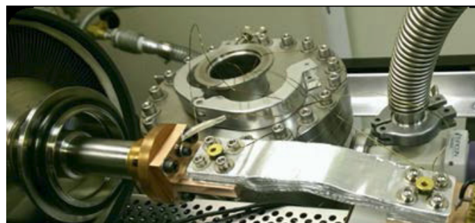
Figure 7.2: Thermal Management Technologies Aluminum thermal strap test. Image Courtesy of Thermal Management Technologies (2015).
