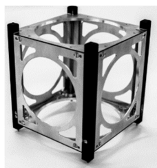
Figure 6.3: 1U CS Structure. Image courtesy of Clyde Space.
