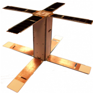
Figure 9.5: SNaP spacecraft with Haigh-Farr's deployable UHF Crossed Dipole antenna. Image courtesy of Haigh.
