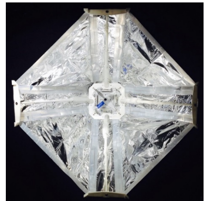
Figure 7.1: End view of Sunshield on CryoCube-1 developed at Sierra Lobo. Image courtesy of Sierra Lobo (2014).
