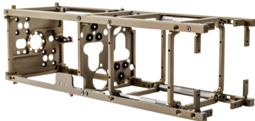
Figure 6.4: NanoAvionics Small Satellite Structures. Image courtesy of NanoAvionics.
