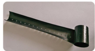
Figure 6.9: The flexible composite member that is employed on the AstroTube. Courtesy of Reveles, et al.
