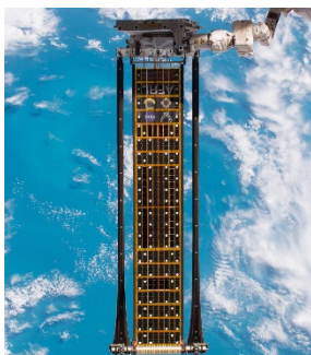
Figure 3.19: Roll-Out Solar Array. Image courtesy of NASA.
