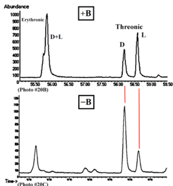
Figure 1. Results of one photo-formose experiment showing the apparent creation of reversible enantiomer excesses. +B and -B refer to opposite magnetic field direction: otherwise, the two runs were performed under nearly identical conditions. Each of the reaction mixtures were subjected to post-reaction oxidation ( H_2O_2 ) to convert a portion of the (several) produced sugars to sugar acids, e.g., erythronic acid and threonic acid. Several other compounds (not shown) are also present.
