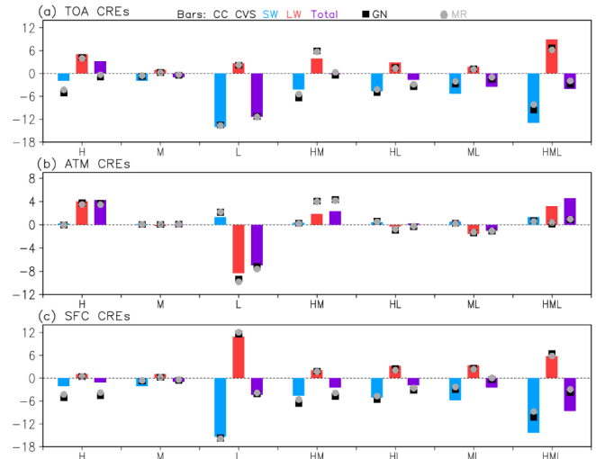
Figure 5. As Fig. 4, but for all-sky (RFO-weighted) CREs.
