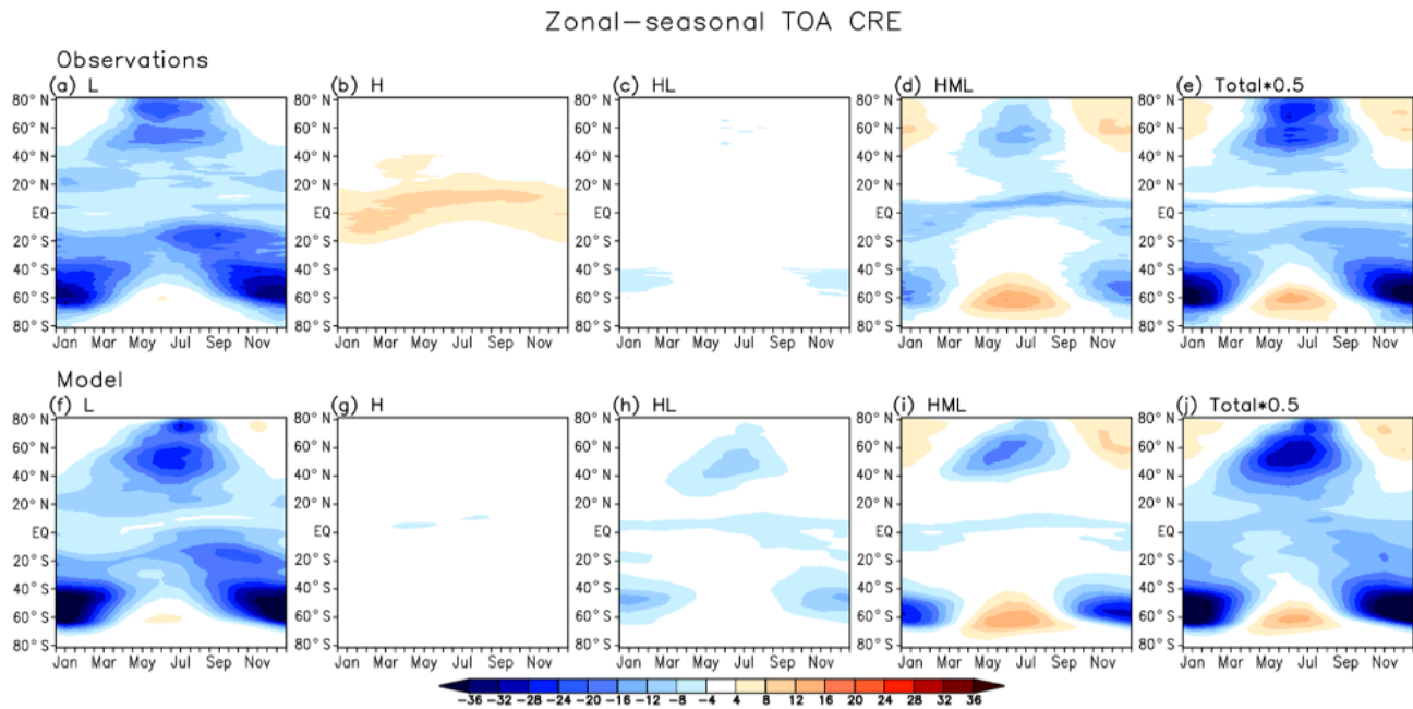
Figure 7. Comparison of the multiyear annual cycle of TOA total (SW + LW) all-sky CRE zonal averages ( \text{W m}^{-2} ) between observations (top row, panels a to e ) and the model (bottom row, panels f to j ) when employing the GN overlap assumption for the four CVS classes with the greatest all-sky CREs according to Fig. 5. The rightmost panels displays the scaled (half) total CRE of all CVS classes combined.
