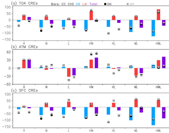
Figure 4. Comparison between observations and the model (GN and MR) of global overcast CREs ( \text{Wm}^{-2} ): top of the atmosphere (TOA) (a), surface (SFC) (c), and atmospheric column (ATM) (b) derived as the difference between the TOA and SFC CREs. CREs are distinguished into shortwave (SW) and longwave (LW) components, and their sum, the “total” CREs for each CVS class, are also shown. Note that the y-axis range is the same for TOA and SFC CRE, but it is substantially more compressed for ATM CRE.
