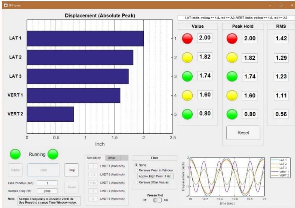
Figure 7: Hydraulic Shaker Displacement Monitor Interface
