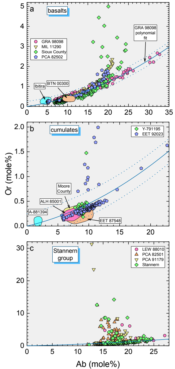
Figure 1. Or vs. Ab plots for select eucrites and eucrite-type achondrites. Note differences in scales.
