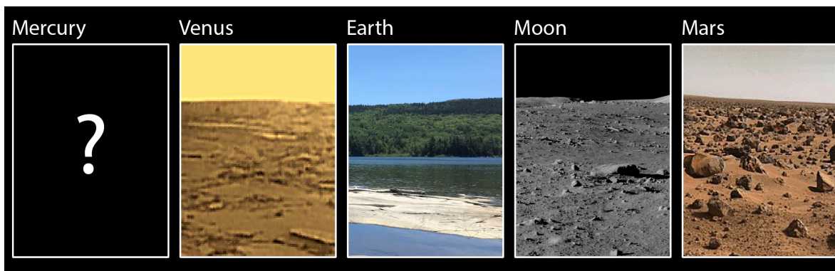
Figure 1. Mercury is the only major terrestrial body for which in situ surface data are lacking, yet the planet holds unique value in understanding how rocky worlds form and evolve.
