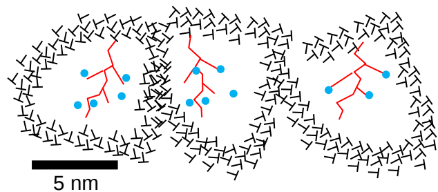
Fig. 1. Illustration of nanoscale sub-grain development at an intermediate stage of solar wind ion damage in olivine, with generation of point defects (blue) by ion collision cascades (red).
