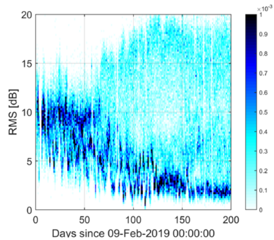
Figure 2 Evolution of the background noise: time-dependent PDF of the displacement noise RMS amplitude, in dB with respect to the lowest value observed up to the end of August 2019, namely 3.2 \times 10^{-12} m .
