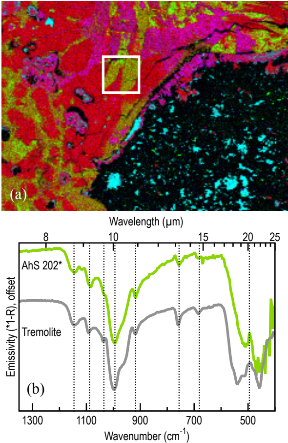
Figure 2. (a) Location of targeted spectral measurement on colorized X-ray map of AhS 202. Red=Mg, Green=Ca, Blue=Al, Cyan=S. White box denoting spectral measurement area is 50 x 50 μm. (b) Spectral measurement from AhS 202 and terrestrial tremolite.
