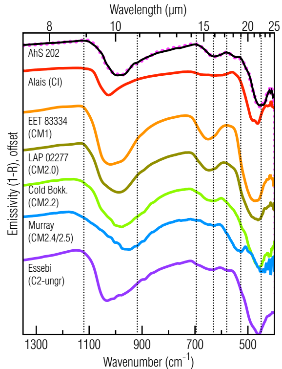
Fig. 1. Average AhS 202 (black) and modeled spectra (dotted pink) compared to CC. Non-AhS sample spectra from [8]. Vertical lines denote key features in AhS 202.
