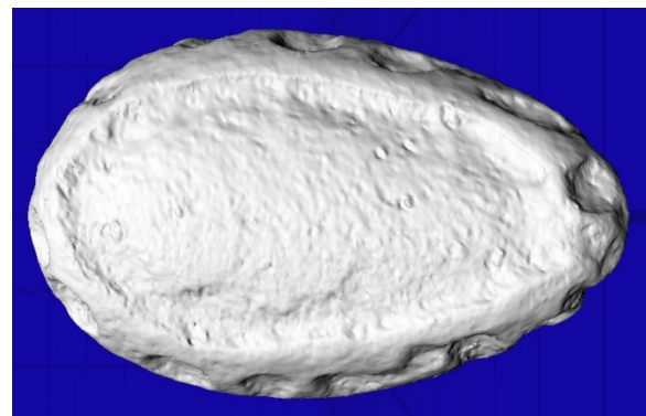
Figure 2: Laser 3D image of DOM 14170, a flight oriented iron meteorite; length of sample is approximately 7 cm.
