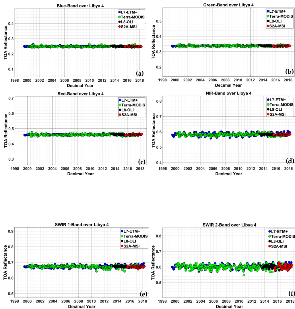
Figure 5. Temporal trend of BRDF-corrected Scaling Adjusted TOA reflectance over Libya 4 site (L7 ETM+, Terra MODIS, L8-OLI, S2A-MSI) in (a) blue band; (b) Green band; (c) Red band; (d) NIR band; (e) SWIR 1 band; (f) SWIR 2 band.
