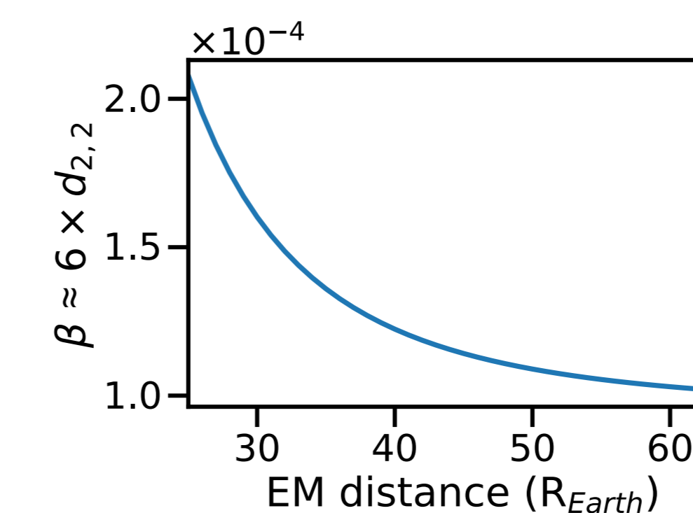
Fig. 4: Core ellipticity with EM distance [6,9]
