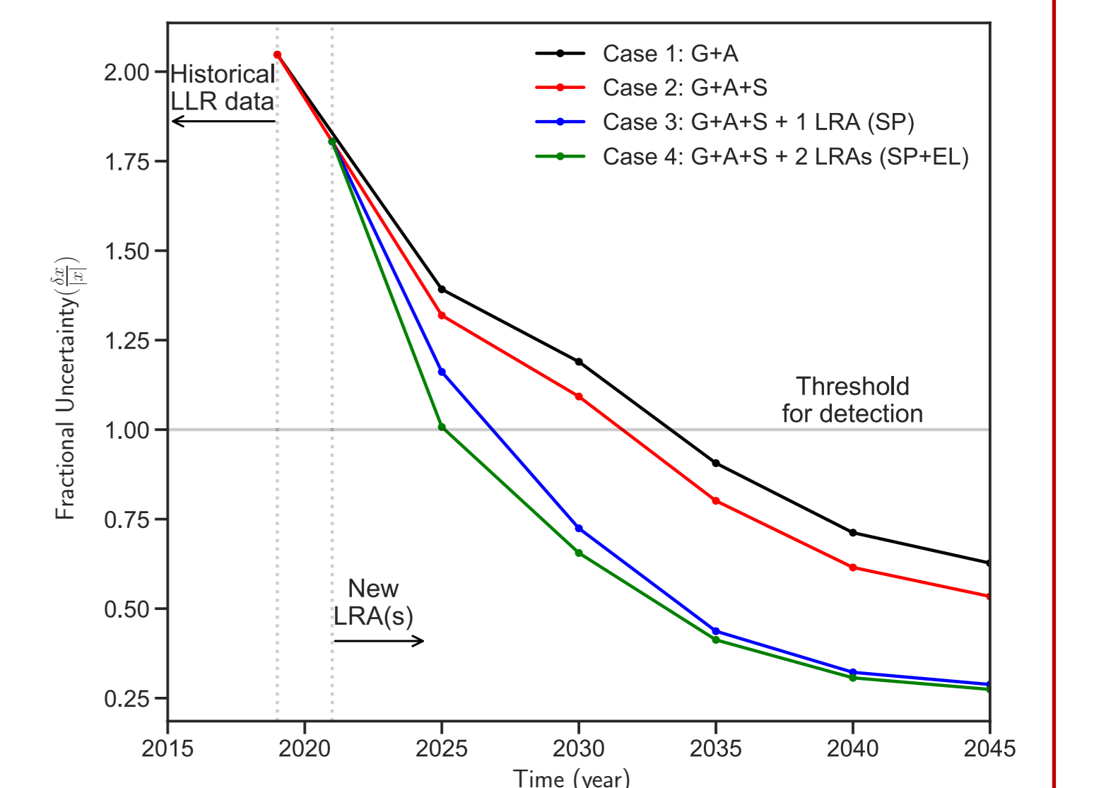
Fig. 6: Recovering the lunar core equatorial ellipticity
