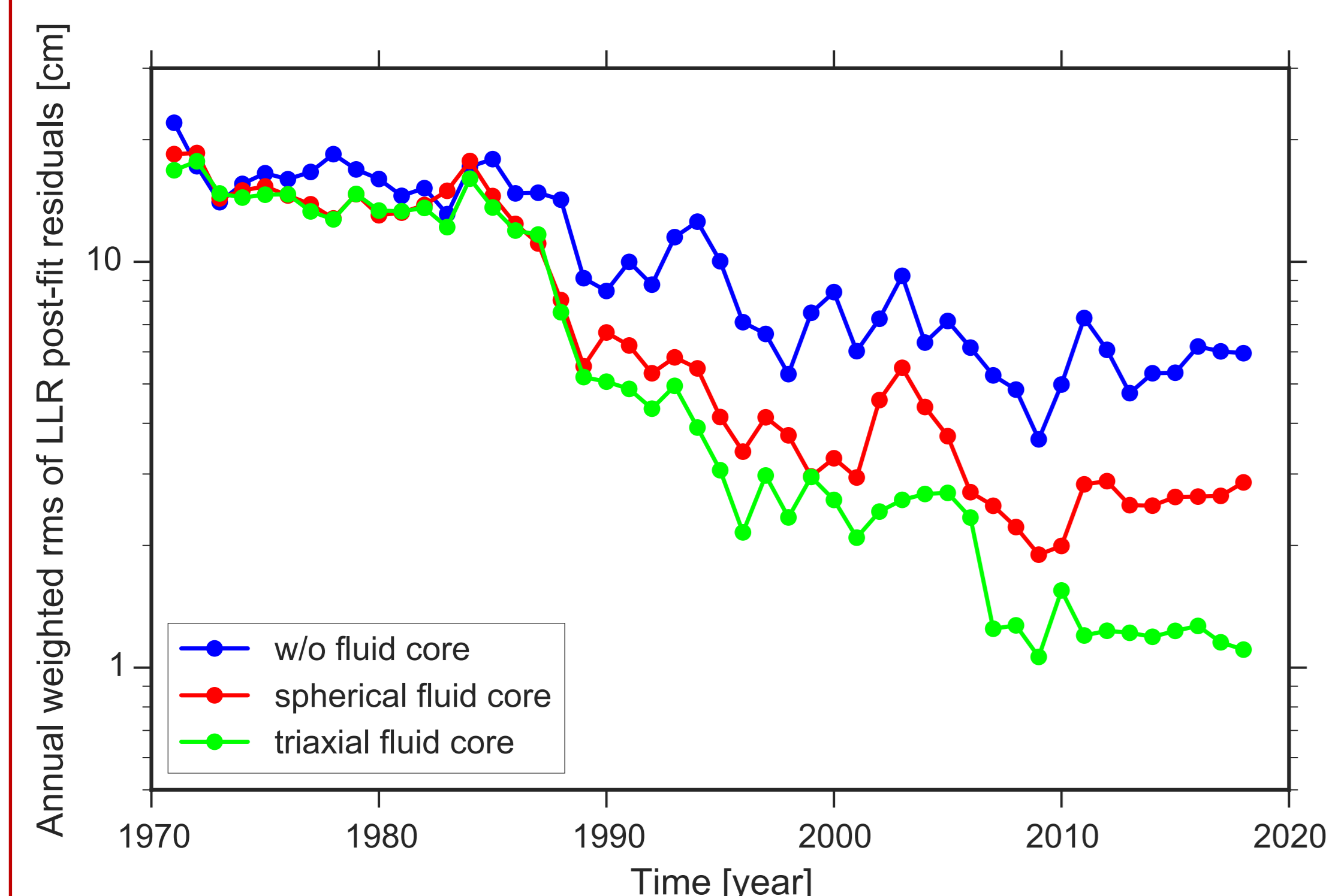
Fig. 3: LLR post-fit residuals (1-way light time). Blue - Model without a fluid core; Red - Model with a spherical fluid core; Green - Model with a triaxial fluid core [5] .
