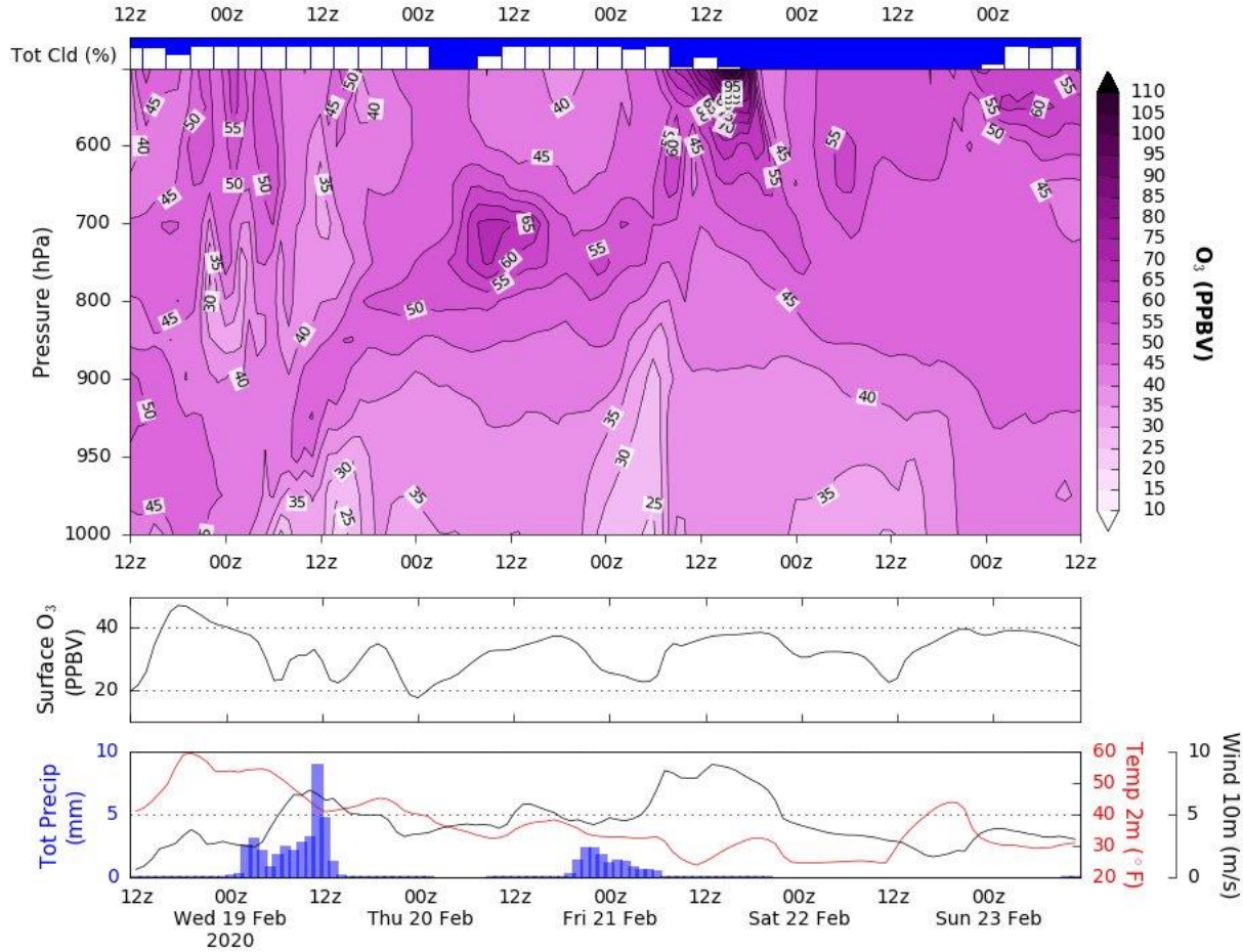
GEOS CF Forecast Initialized on 12z 02/18/2020
