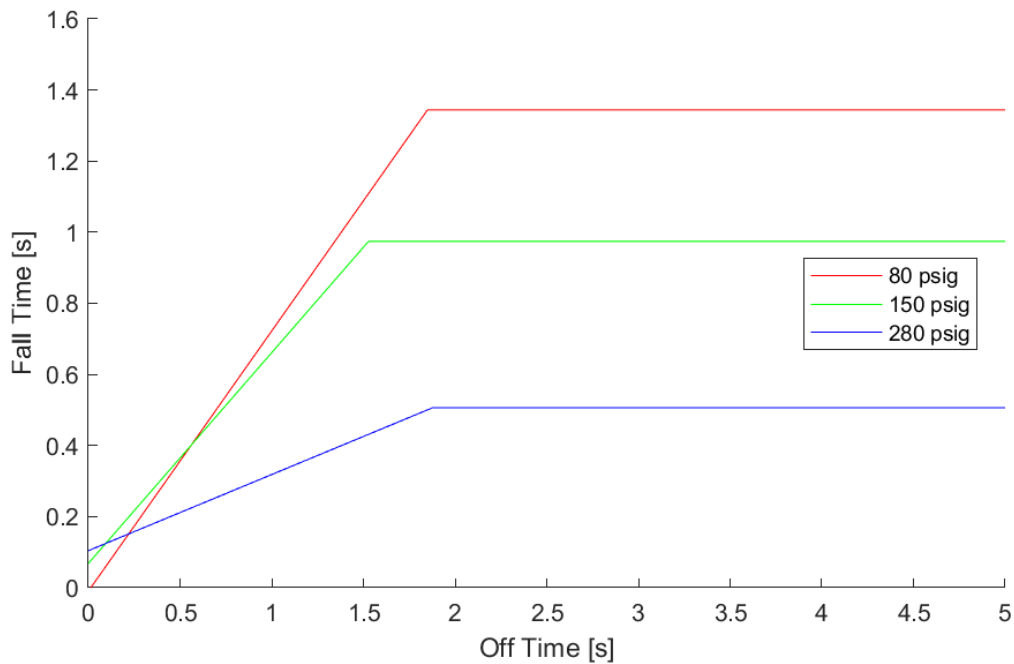
Figure 10. Linear best fit lines for the average fall time taken from Figure 4, Figure 6, and Figure 8 against the off time for tested reservoir head pressures in phase 1.
