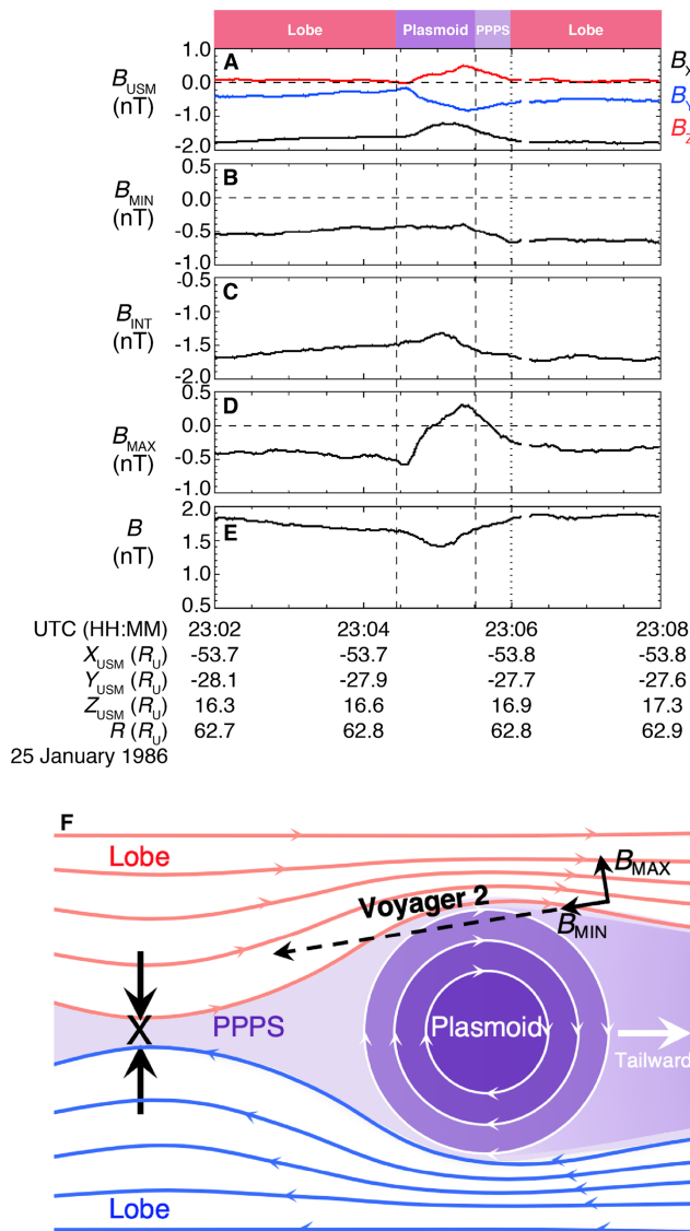
Figure 3. (a–e) Voyager 2 magnetic field data during the plasmoid encounter shown in (a) USM coordinates and (b–d) minimum variance analysis coordinates. The vertical dashed lines mark the plasmoid signature and are implemented for the minimum variance analysis interval. The postplasmoid plasma sheet (PPPS) is denoted as the region between end of the plasmoid (second vertical dashed line) and the vertical dotted line. (f) Schematic showing the Voyager 2 trajectory through the plasmoid and PPPS in Uranus' magnetotail as suggested by magnetic field signatures. Red and blue field lines represent the -B_{X,USM} and +B_{X,USM} tail lobes, respectively. The purple shaded region illustrates the central plasma sheet. The vertical black arrows indicate the open field line motion towards the current sheet with an "X" marking the location of the reconnection X-line. The horizontal white arrow demonstrates the tailward direction of the plasmoid after it has been ejected via magnetic reconnection.
