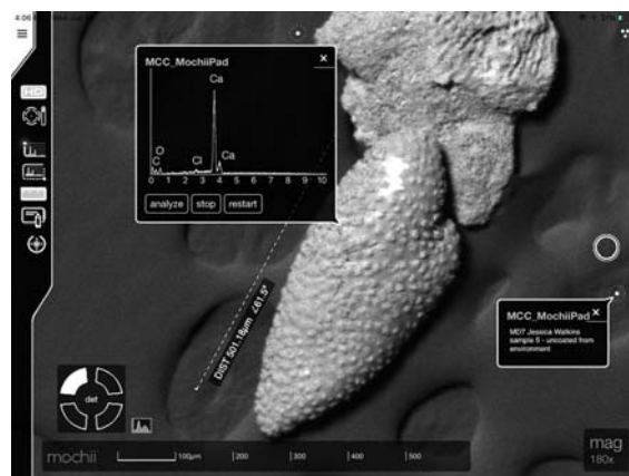
Figure 3. Spectroscopy and image of sediment particle gathered on EVA and analyzed in-situ in the underwater Aquarius habitat by NEEMO XXIII crew member J. Watkins. Some sediment contained calcium carbonate from deceased organisms, whereas others (not shown) were silicate-based.
