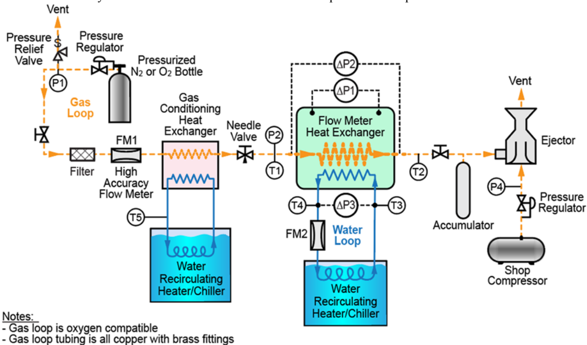
Figure 6. Test setup to measure FMHX performance during low-pressure operation.
