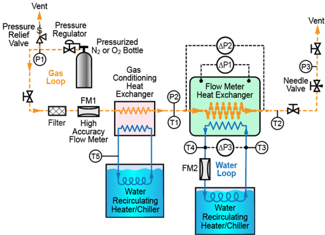
Figure 8. Test setup to measure FMHX performance during high-pressure operation.
