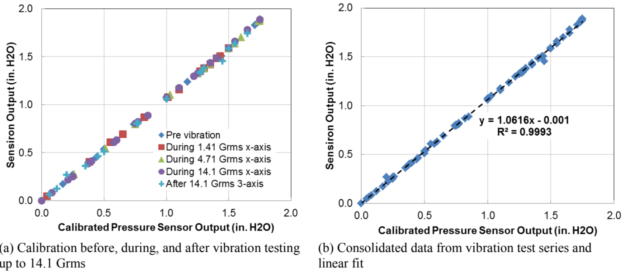
Figure 15. The Sensirion transducer is highly linear and insensitive to vibration. Note 1 in. H 2 O = 248 Pa.
