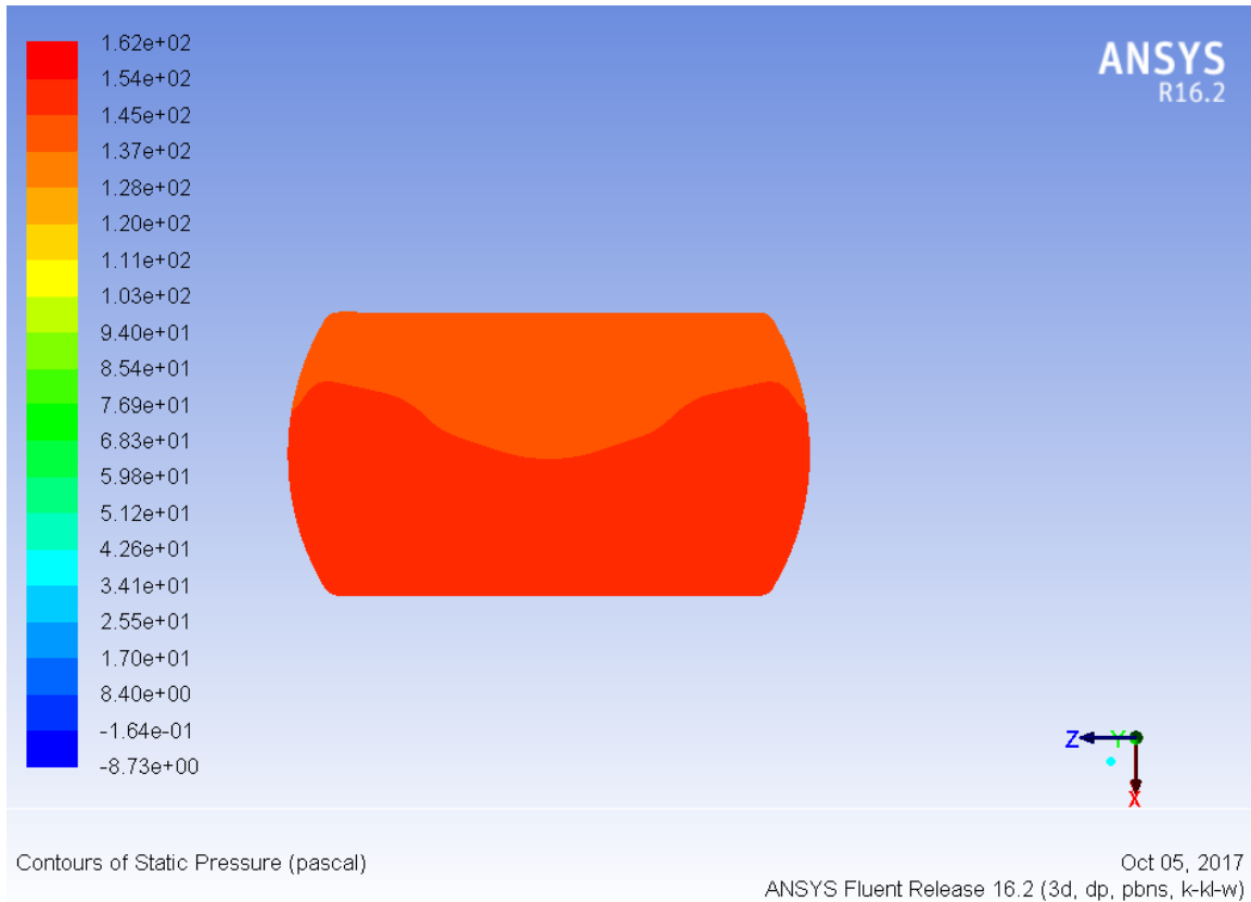
Figure 4. CFD predicts very little variation in static pressure across the inlet face of the microtube array.
