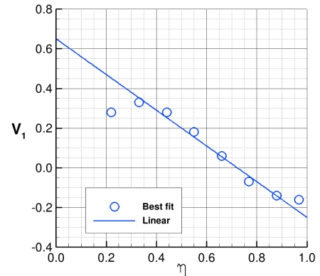
Figure 8. Spanwise distribution of V_1 from best-fit procedure.
