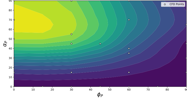
Fig. 9 The values for the first ROM coefficient for pressure across \alpha_P and \phi_P for the core of the Block 1B crew vehicle. The dots represent locations of CFD points.
