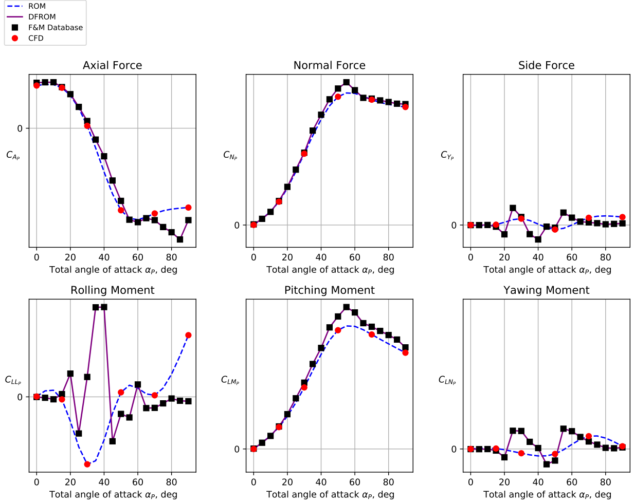
Fig. 17 Comparison of ROM force and moments to DFROM versus angle of attack at \phi_P = 0^\circ for the Block 1B crew vehicle.
