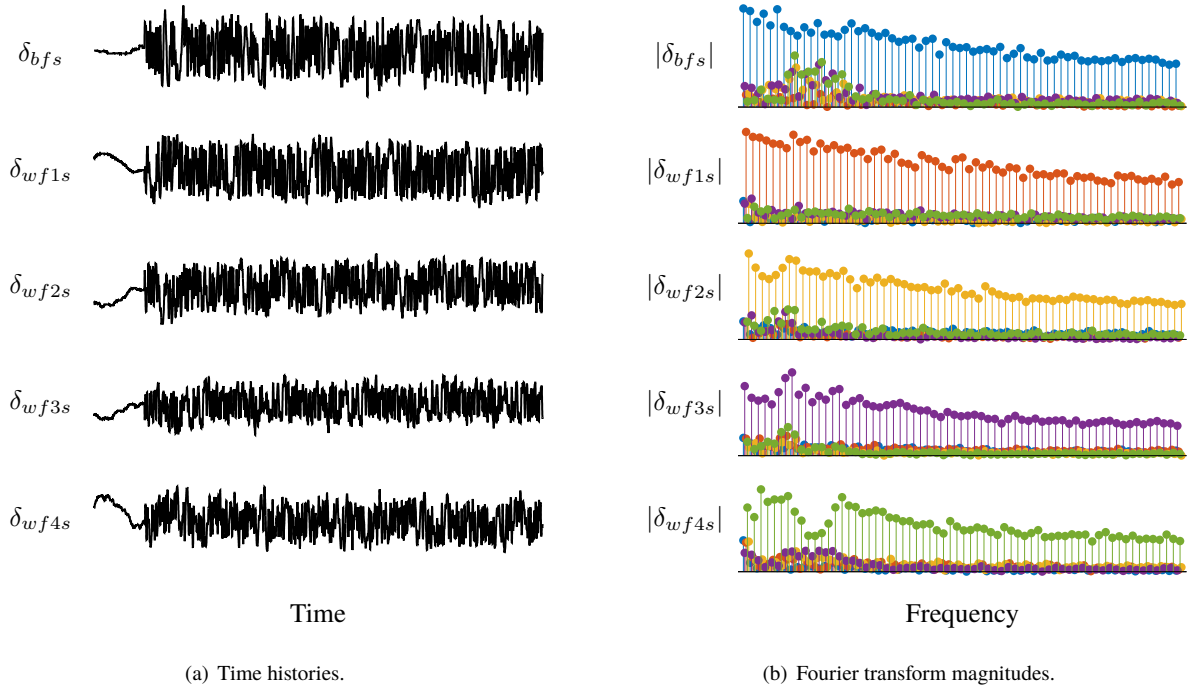
Fig. 14 X-56A measured input data.
