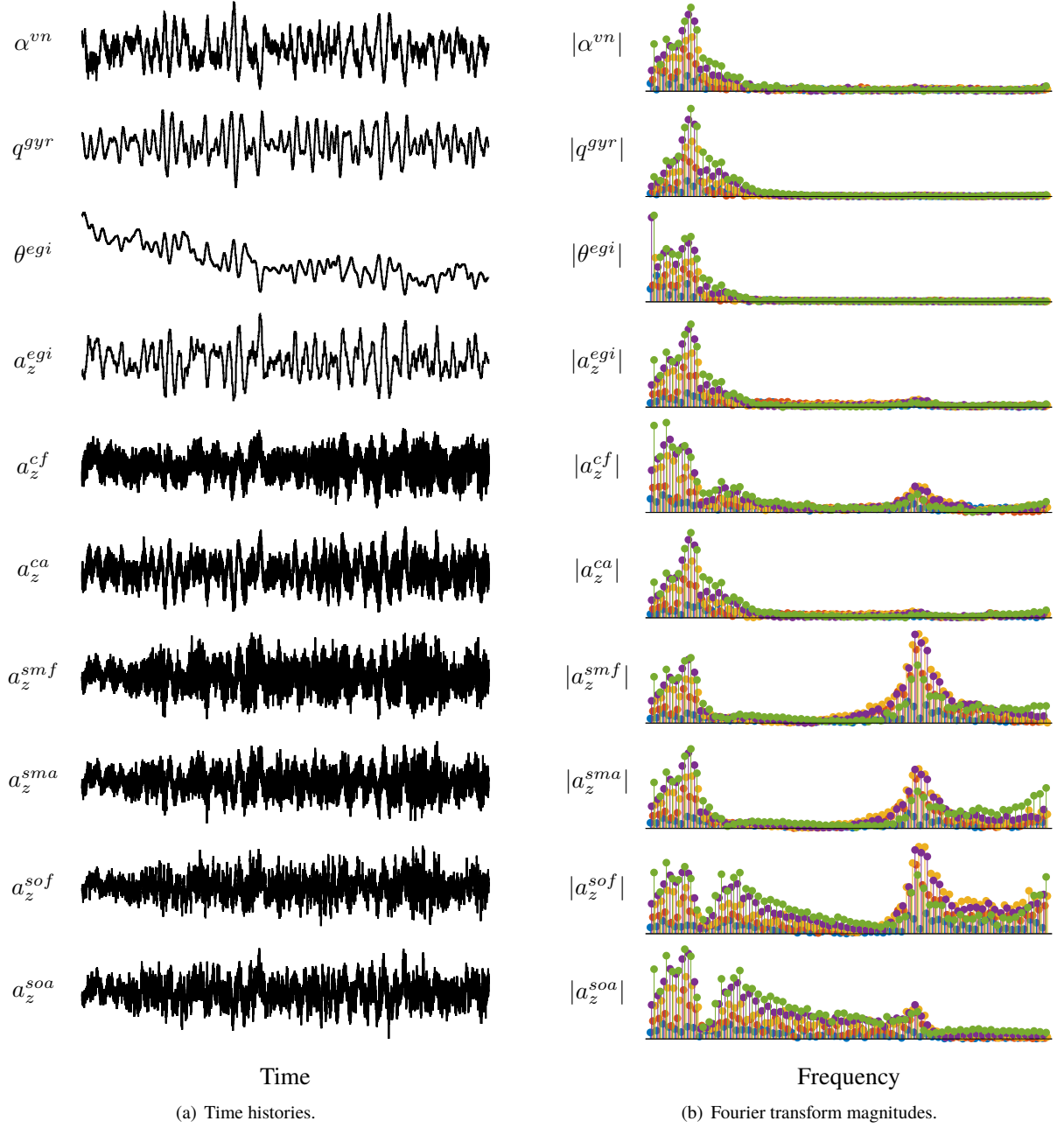
Fig. 16 X-56A measured output data.
