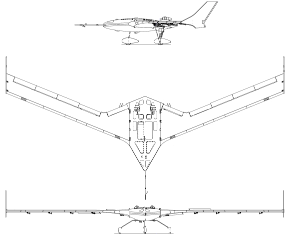
(b) Three-view drawing schematic.
