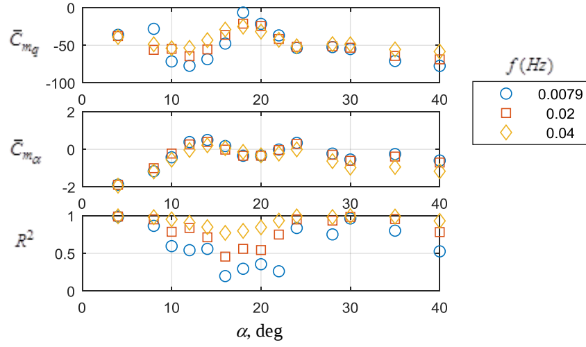
Figure 5b. Harmonic analysis of C_m using first-order model and data from CFD forced oscillations in pitch for three frequencies, \alpha_A=5^\circ , GTT model.
