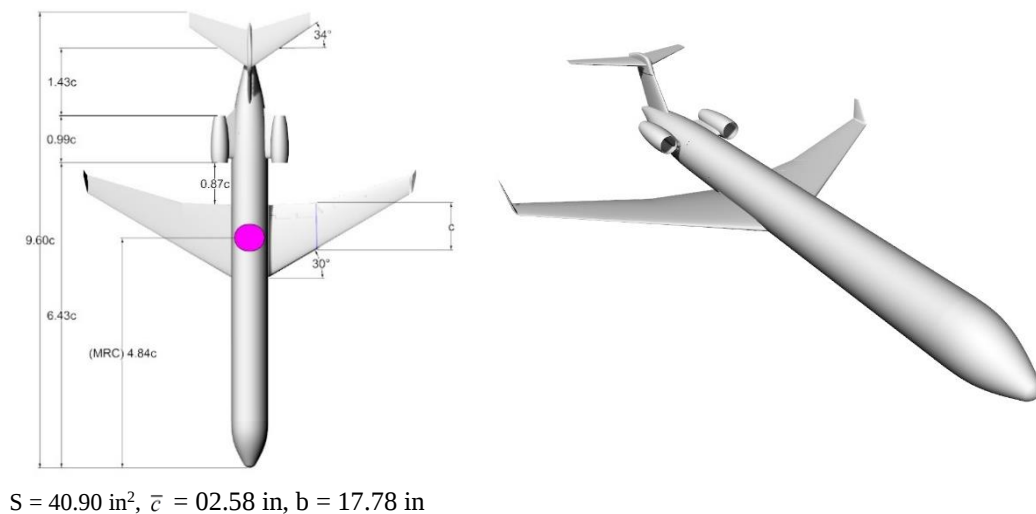
Figure 1. GTT model geometry and perspective view.
