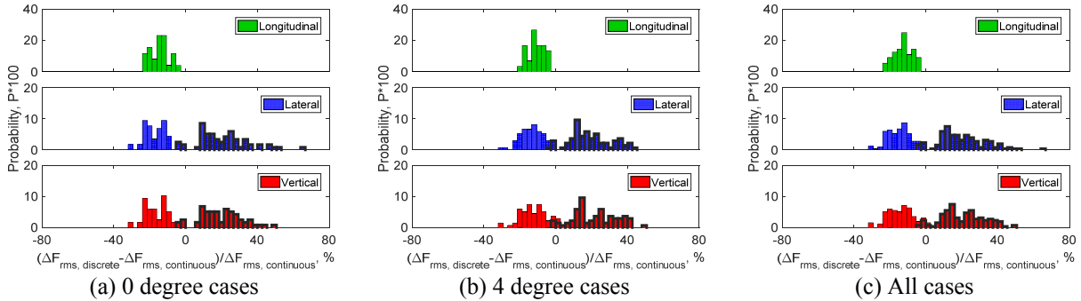
Figure 8. Histogram of percent difference in BFF \Delta F_{rms} based on continuous integration and 16 vPTs/ring.
