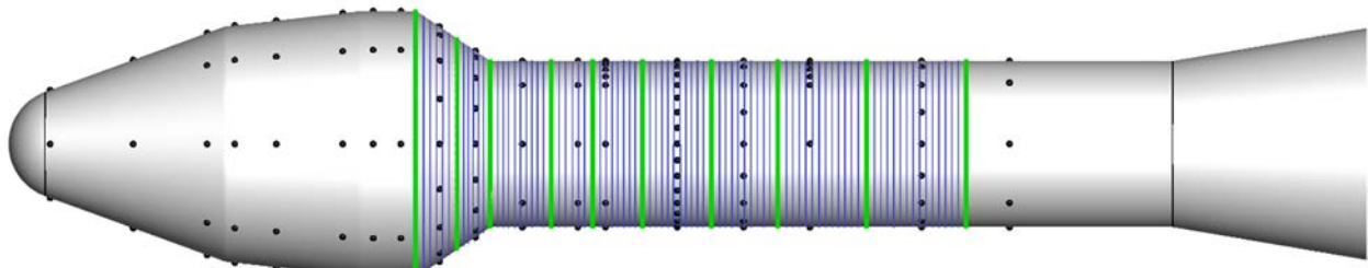
Figure 26. Longitudinal integration boundaries for increased longitudinal sensor density.
