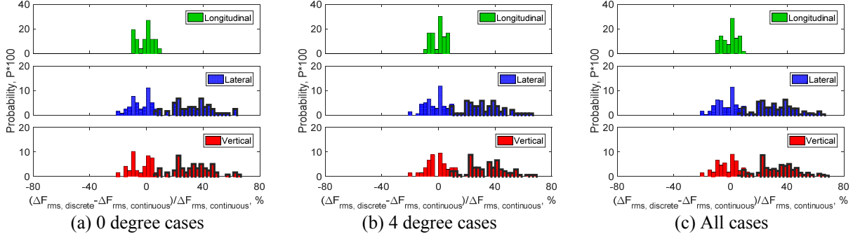
Figure 9. Histogram of percent difference in BFF \Delta F_{rms} based on continuous integration and 32 vPTs/ring.
