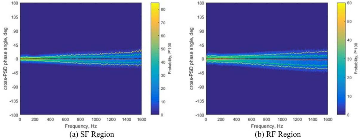
Figure 24. Histogram of phase of BFF CPSD(continuous, 16 vPTs/ring).
