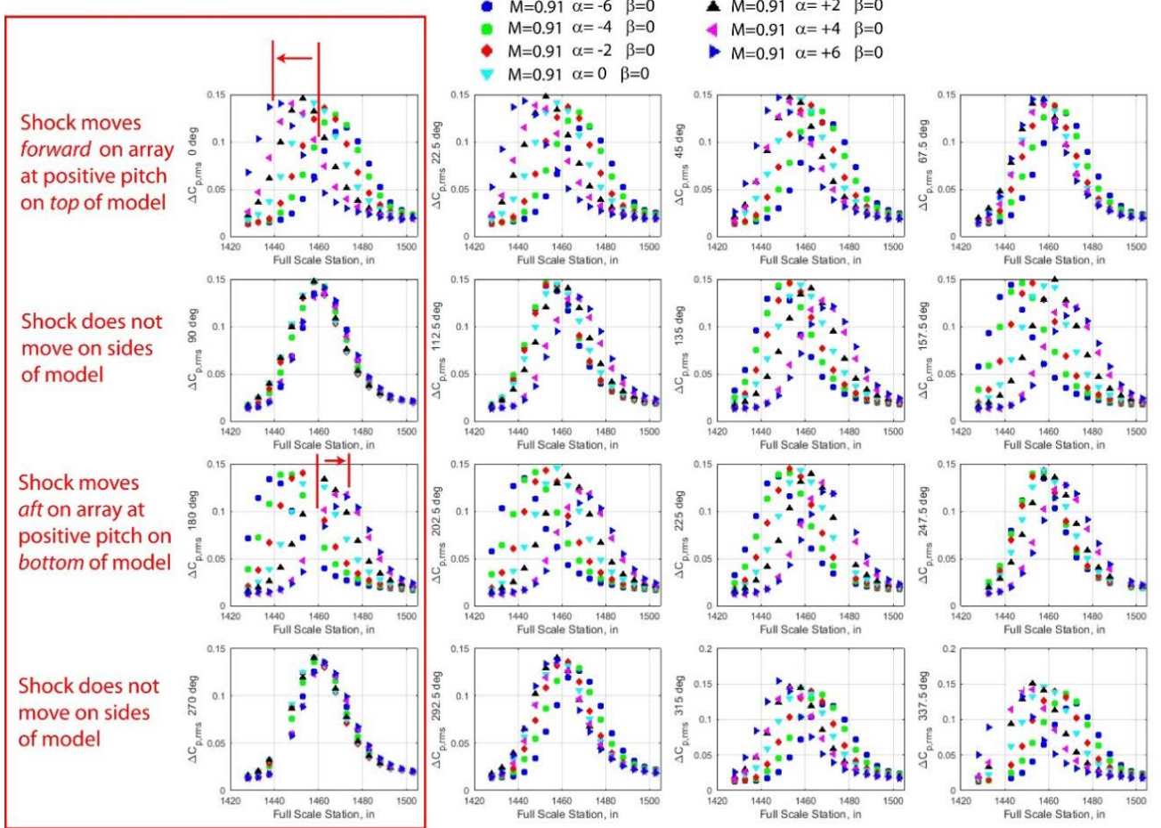
Figure 19. \Delta C_{p,rms} on the 16 shock arrays at a Mach number of 0.91 and \alpha=-6^\circ to +6^\circ , and \beta=0^\circ .
