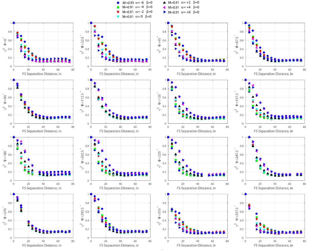
Figure 28. Longitudinal magnitude-squared coherence ( \gamma^2 ) between port 'a' and each subsequent port versus full-scale sensor separation distance at a Mach number of 0.91 and \alpha = -6^\circ, -4^\circ, -2^\circ, 0^\circ, +2^\circ, +4^\circ , and +6^\circ and \beta = 0^\circ at each azimuthal shock sensor array.
