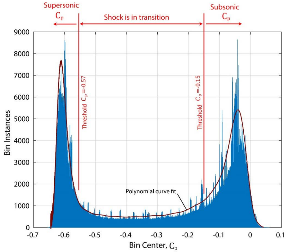
Figure 21. Summed histogram of pressure coefficient for all 16 sensor ports (a through p) on the shock array at \Psi=90^\circ for a Mach number of 0.91 and \alpha=0^\circ and \beta=0^\circ with supersonic and subsonic threshold C_p values identified.
