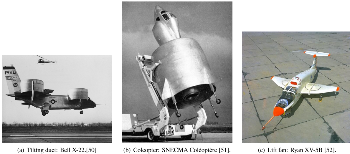
Fig. 6 Historical ducted propeller aircraft.
