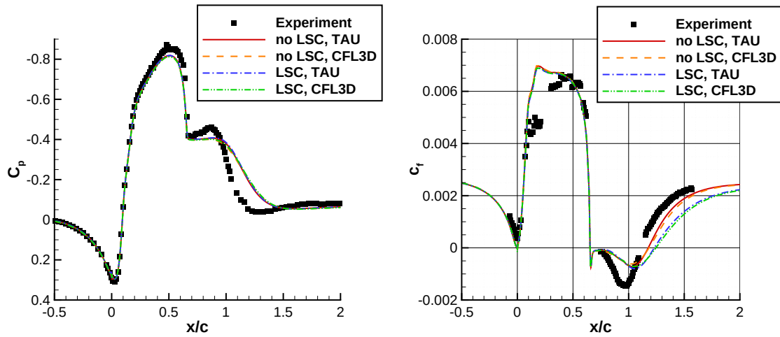
Figure 5. NASA-hump. Pressure distribution (left) and skin-friction distribution (right). SSG/LRR- \omega with and without length-scale correction (LSC) compared to experimental data by Greenblatt et al. 24–26
