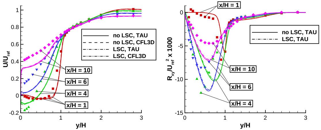
Figure 3. Backward-facing step. Velocity profiles (left) and Reynolds-shear stress profiles (right). SSG/LRR- \omega with and without length-scale correction (LSC) compared to experimental data by Driver and Seegmiller 23 (symbols).
