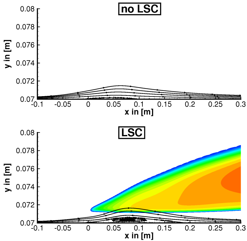
Figure 11. Axisymmetric separation. Recirculation region with and without length-scale correction in shaded area. TAU solution.
