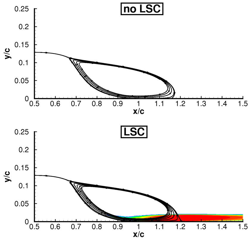
Figure 6. NASA-hump. Recirculation region with and without length-scale correction in shaded area. TAU solution.
