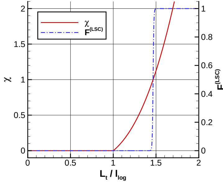
Figure 1. Parameter \chi for modifying the \omega -destruction term according to the Yap correction and length-scale correction function F^{(LSC)}(\chi) , both plotted versus the length-scale ratio L_t / \ell_{\log} .
