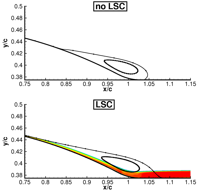
Figure 9. Axisymmetric bump. Recirculation region with and without length-scale correction in shaded area. TAU solution.
