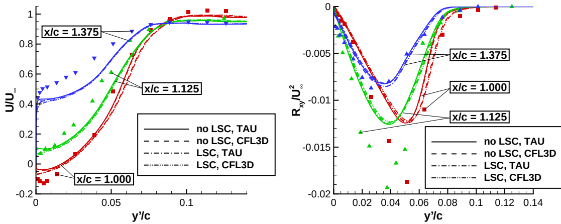
Figure 8. Axisymmetric bump. Velocity profiles (left) and Reynolds-shear stress profiles (right). SSG/LRR- \omega with and without length-scale correction (LSC) compared to experimental data by Bachalo and Johnson 27 (symbols).
