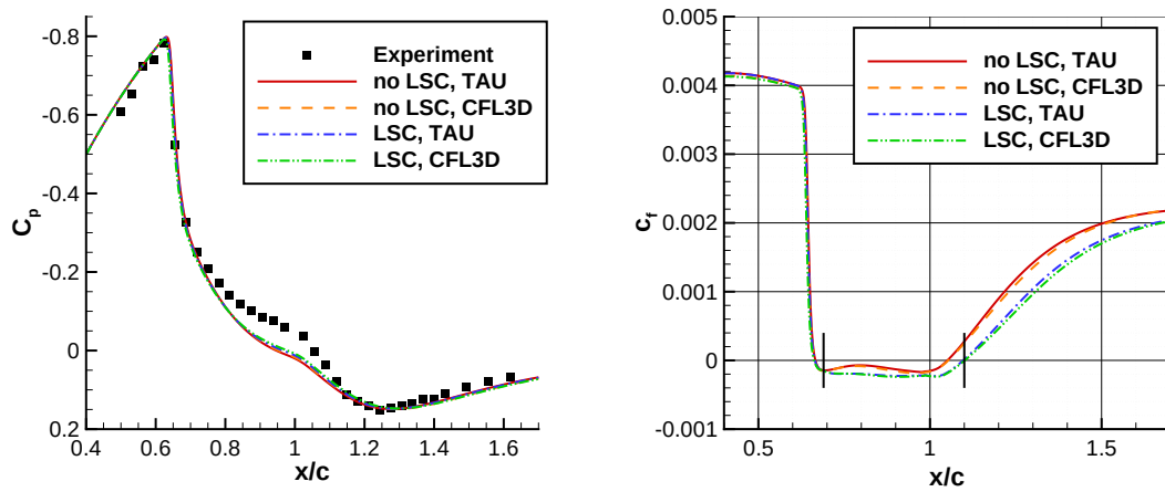
Figure 7. Axisymmetric bump. Pressure distribution (left) and skin-friction distribution (right). SSG/LRR- \omega with and without length-scale correction (LSC) compared to experimental data by Bachalo and Johnson. 27
