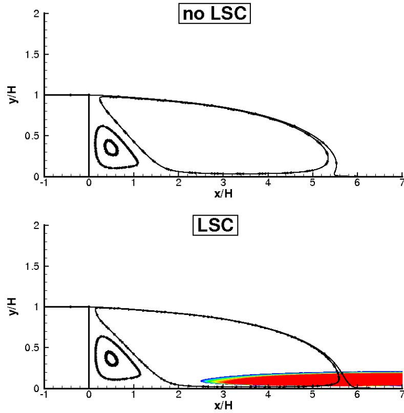
Figure 4. Backward-facing step. Recirculation region with and without length-scale correction in shaded area. Steady-state TAU solution.
