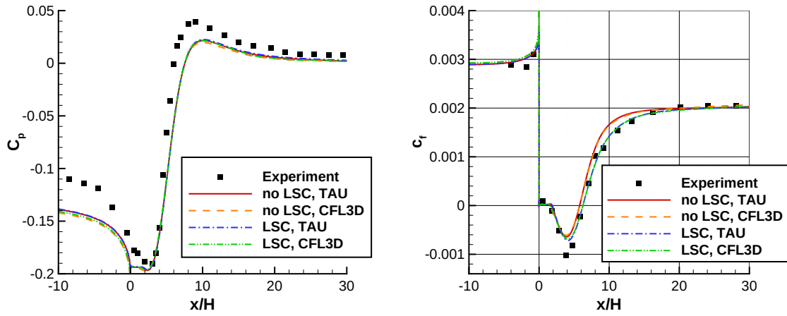
Figure 2. Backward-facing step. Pressure distribution (left) and skin-friction distribution (right). SSG/LRR- \omega with and without length-scale correction (LSC) compared to experimental data by Driver and Seegmiller. 23
