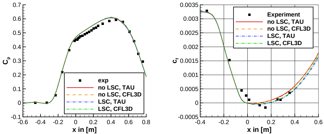
Figure 10. Axisymmetric separation. Pressure distribution (left) and skin-friction distribution (right). SSG/LRR- \omega with and without length-scale correction (LSC) compared to experimental data by Driver. 28
