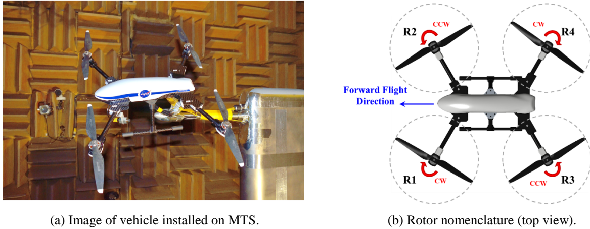
Figure 1: The SUI Endurance quadcopter.
